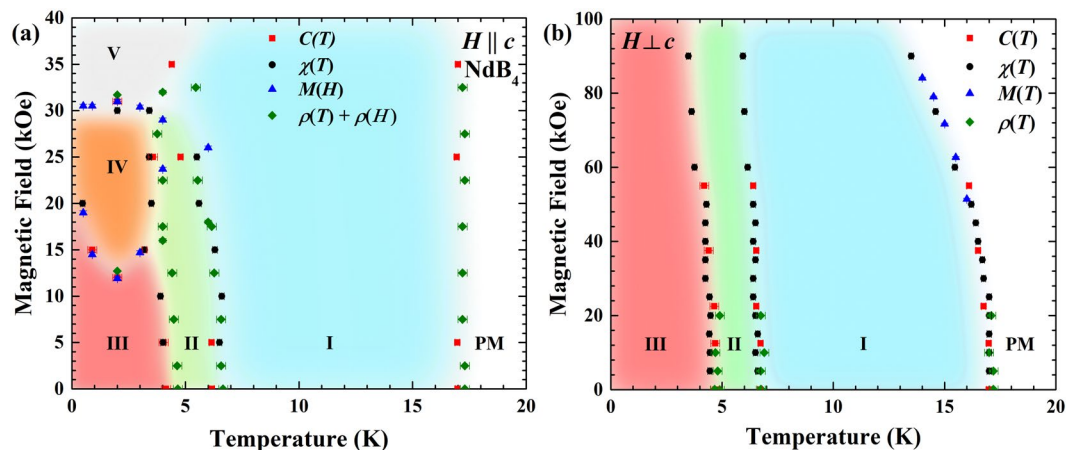
Figure 5. Magnetic phase diagrams of \text{NdB}_4 for (a) H \parallel c and (b) H \perp c . For both field directions, Phase I corresponds to a non-collinear antiferromagnetic order, while Phases II and III are two different incommensurate structures. Phases IV and V for H \parallel c correspond to the \frac{1}{5} -magnetisation plateau and the fully polarised state respectively.
