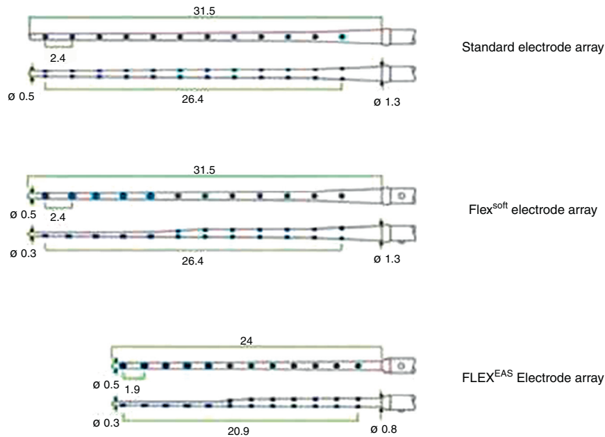
Figure 2 Schematic representation of MED-EL FLEX™ EAS (21 mm) electrode. Standard electrode array.
