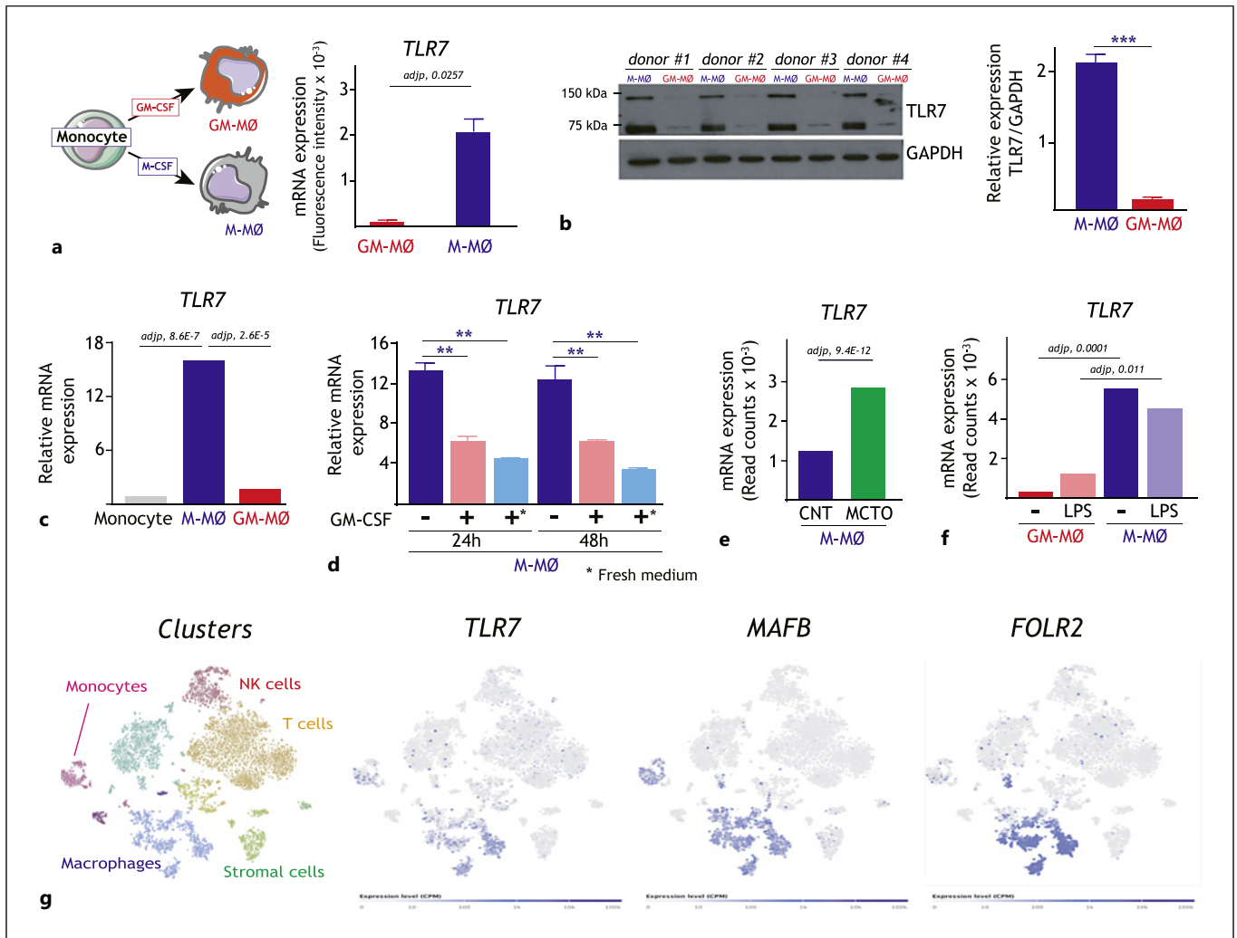
Fig. 1. Regulated expression of TLR7 in human macrophages. a Schematic representation of the in vitro generation of M-MØ and GM-MØ from peripheral blood monocytes. TLR7 gene expression (normalized fluorescence intensity) in M-MØ and GM-MØ, as determined in microarray experiments (GSE68061) on three independent samples. Statistically significant differences (adjp) are indicated. b TLR7 protein levels in four independent preparations of M-MØ and GM-MØ, as determined by Western blot (left panel). Relative level of TLR7 , including both the full-length (140 kDa) and the proteolytically processed mature (75 kDa) forms, were determined in M-MØ and GM-MØ by densitometry. Mean \pm SEM of four independent samples is shown (*** p < 0.001). c Relative TLR7 gene expression in Monocytes, M-MØ and GM-MØ, as determined by RNA-sequencing (GSE188278) on three independent samples. Statistically significant differences are indicated. d TLR7 gene expression in M-MØ before and after exposure to GM-CSF (1,000 U/
