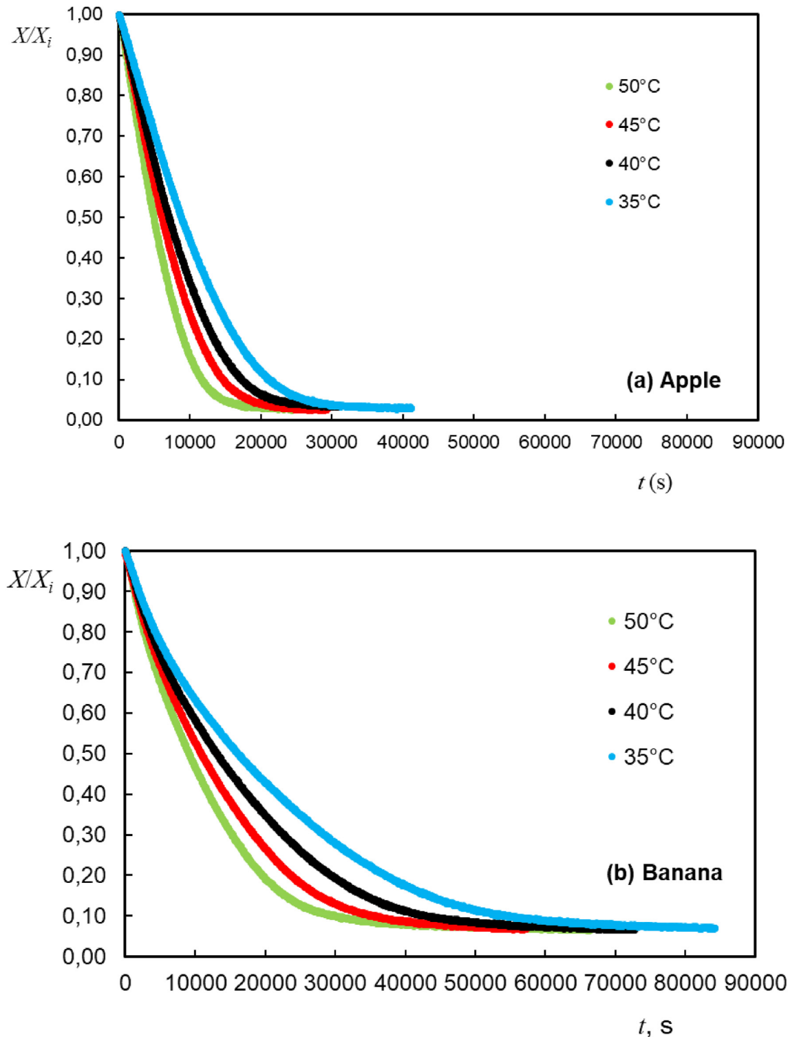
Figure 2. Dimensionless moisture content evolution during drying carried out with the air-drying stream ( 1.6 \text{ m s}^{-1} ) at different temperatures for: (a) Bravo de Esmolfe apple samples and (b) Madeira banana samples.
