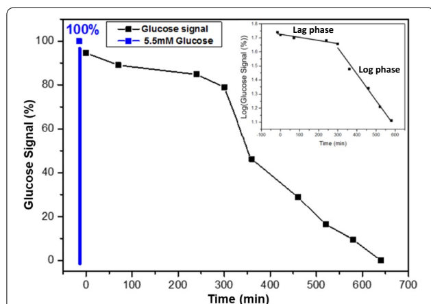
Fig. 3 Monitoring of the metabolic activity of bacterial biofilm. The metabolic activity was monitored with the use of a redox-reactive SiNW-FET device and the time-dependence of the glucose signal is shown. First, the biofilm was grown in MSgg medium (glycerol and glutamate) and incubated at 30 °C for 40 h. Then, the MSgg medium was replaced by the glucose-based medium. The bacterial biofilm consumes all the glucose in 11 h. The minimal-broth medium contains 5.5 mM glucose at the beginning of the measurements. Inset: bacterial-growth rate curve presented as the logarithm of glucose signal versus time. The lag phase and log phase of bacterial glucose metabolism are monitored with the use of a redox-reactive SiNW FET
