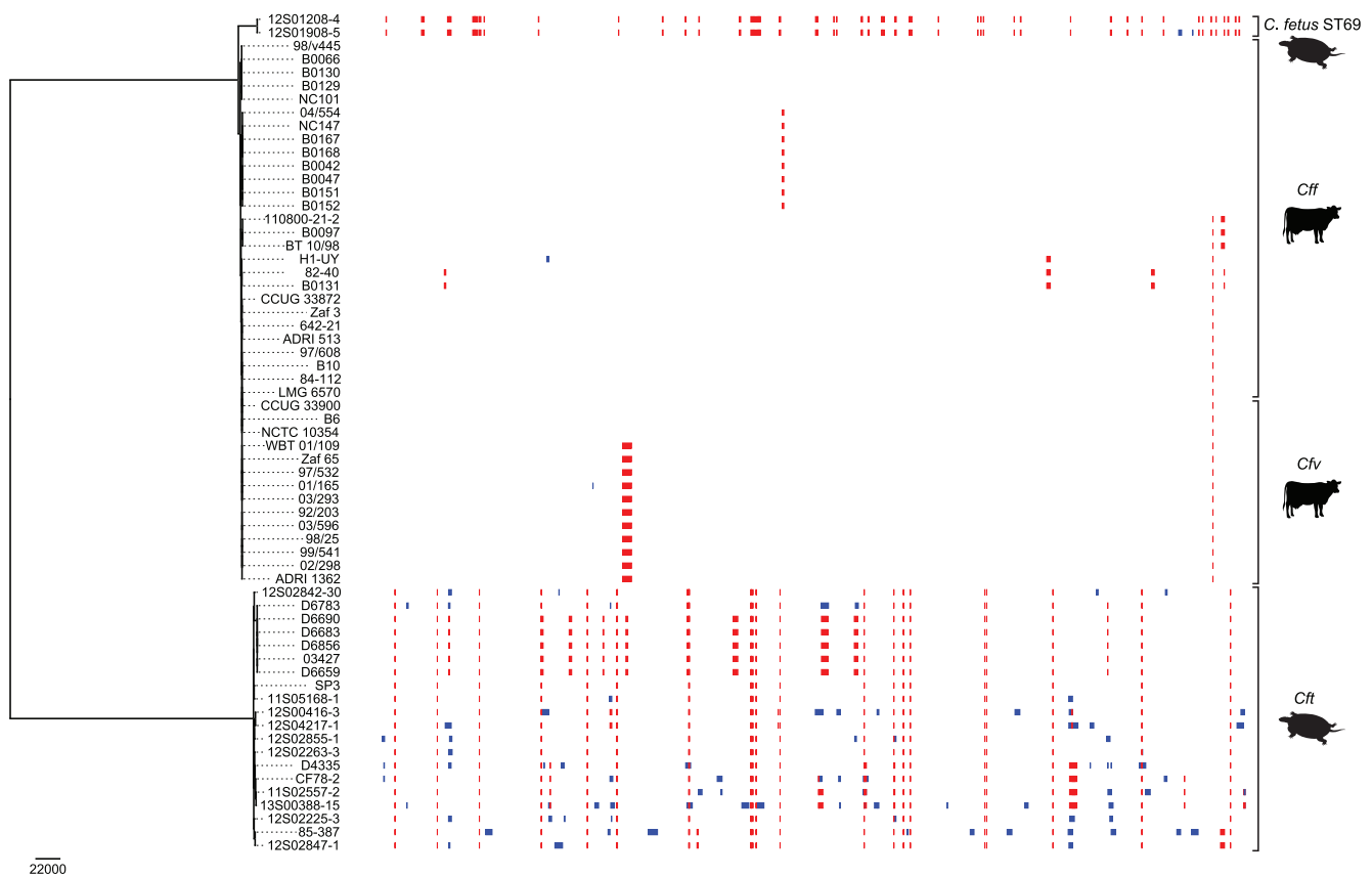
Fig. 1. —Core genome-based phylogeny for Campylobacter fetus . Identical recombination regions in two or more strains are indicated in red; unique recombination regions are indicated in blue. Campylobacter fetus ST69 is associated with reptiles (chelonians), C. fetus subsp. fetus ( Cff ) and venerealis ( Cfv ) are associated with mammals (primarily ungulates), and C. fetus subsp. testudinum ( Cft ) is primarily associated with reptiles.
