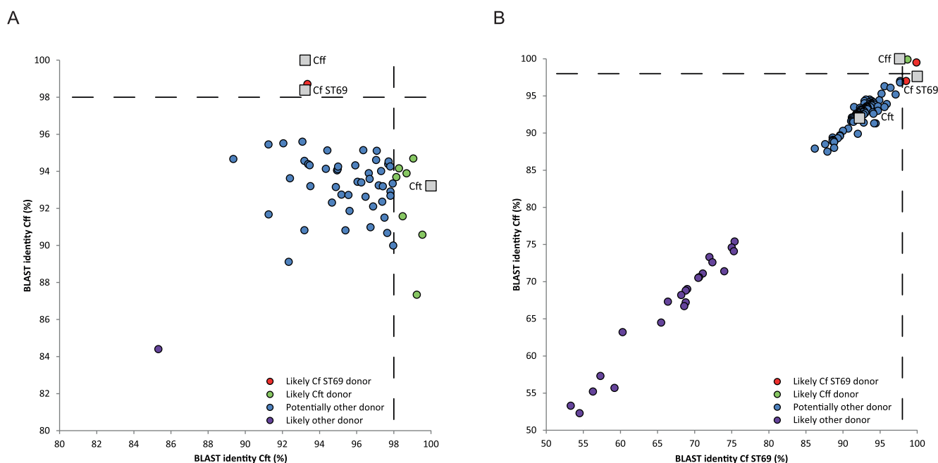
FIG. 2. —Scatter plot based on the BLAST-based nucleotide identities of all recombination regions identified in Campylobacter fetus ST69 ( Cf ST69) isolate 12S01908-5 (A) and all C. fetus subsp. testudinum ( Cft ) strains (B). A BLAST search was performed for each recombination region and the genomes of Cft strain 03-427 and C. fetus subsp. fetus ( Cff ) strain 82-40 (A) and Cff strain 82-40 and Cf ST69 isolate 12S01908-5 (B). The nucleotide identities of the recombination regions are plotted as circles; the nucleotide identities of the reference genomes are plotted as squares. The dashed line shows the \geq 98\% nucleotide identity. x- and y-axis range 80–100% (A) or 50–100% (B).
