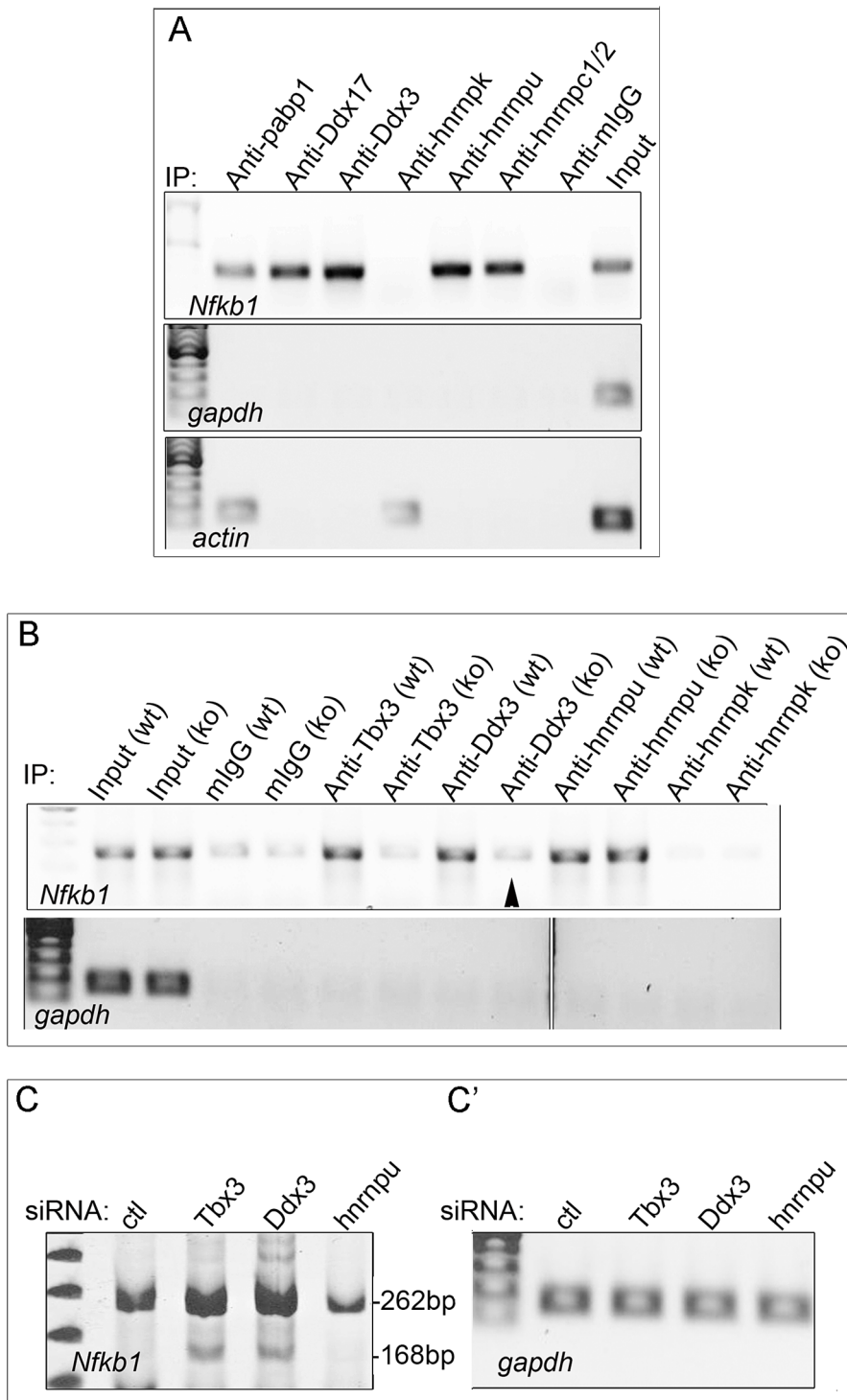
Figure 6. Tbx3 binding partners associate with the Nfkb1 mRNA that is alternatively spliced in response to Tbx3, and a subset require Tbx3 to bind this mRNA. A) RNA-IP with anti-Tbx3 on embryo lysates using antibodies against Tbx3 interacting proteins to test binding to the Nfkb1 transcript which is differentially spliced in response to Tbx3 in mouse limb. Actin and Gapdh are negative controls. Note that not all Tbx3 interactors bind this mRNA. B) RIP/RT-PCR testing Tbx3 interactors for binding of the Nfkb1 mRNA in Tbx3 wild type (wt) and null (ko) murine embryonic fibroblasts (MEFs). Ddx3 requires Tbx3 to bind the Nfkb1 mRNA (arrowhead) but hnrmpu does not. C) RT-PCR assay of splice variants in control, Tbx3 and Ddx3 siRNA knockdown MEFs. Knockdown of Ddx3 results in the same alternative splicing of Nfkb1 exon 11 as Tbx3 knockdown, whereas knockdown of hnrmpu decreases the total amount of Nfkb1 transcript but has no effect on exon 11 splicing. C') Gapdh control RT-PCR. doi:10.1371/journal.pgen.1004247.g006
