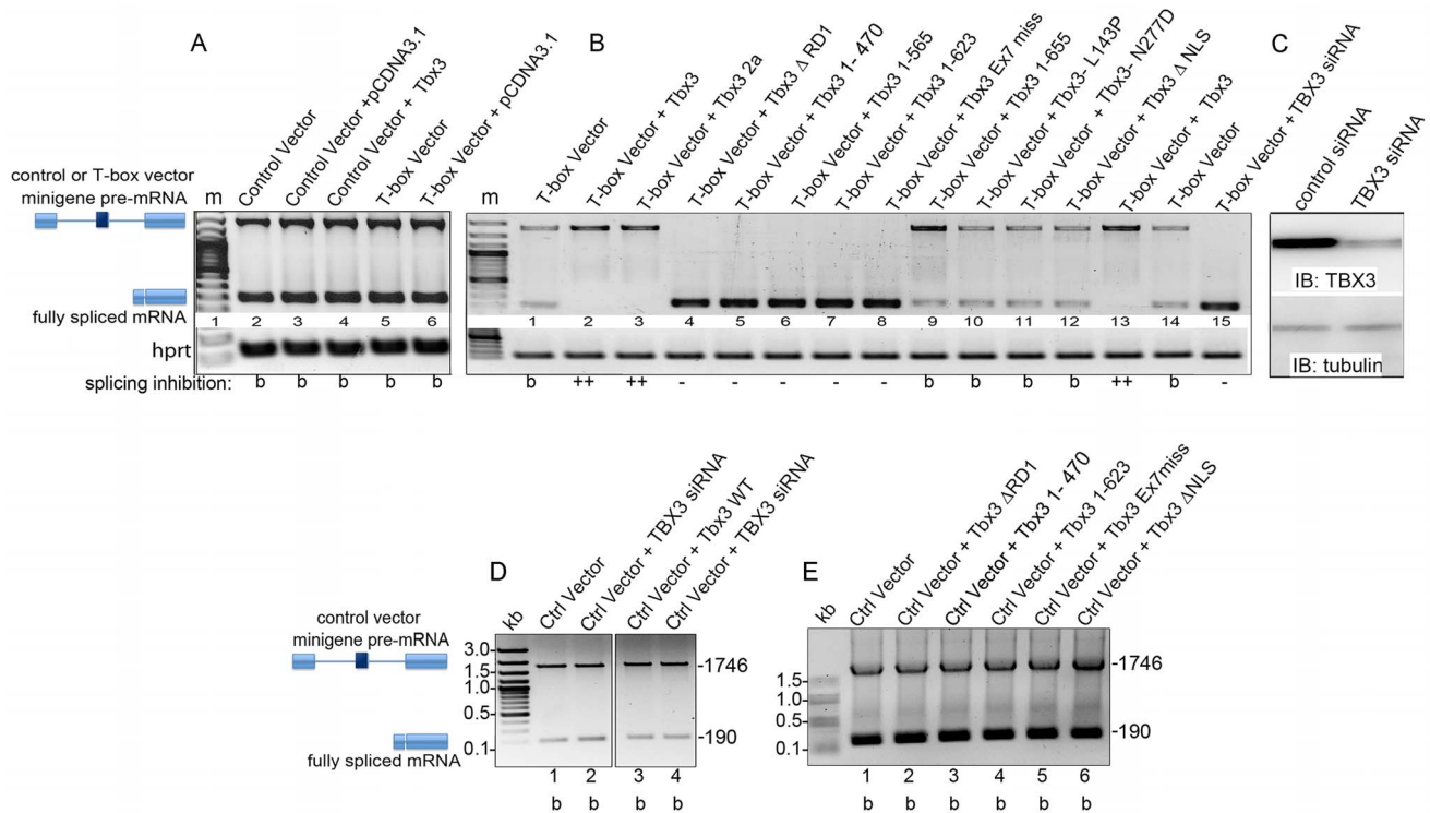
Figure 3. Tbx3 regulates alternative splicing in vitro . A) Either pRHCglo (Control vector) or RHCglo+T-box binding element (T-box vector) were co-transfected into HEK293 cells with Tbx3 expression vectors indicated above each lane. Splicing products were assayed by RT-PCR; positions of unspliced pre-mRNA and spliced products are indicated at left. Hprt control PCR products are shown below. B) Ability of Tbx3 mutant proteins to completely regulate T-box splicing. Symbols at bottom summarize effect on splicing inhibition. b, baseline ratio of pre-mRNA to completely spliced mRNA; +, splicing inhibited over baseline; -, no inhibition. C) Immunoblot of control or TBX3 siRNA lysates probed for TBX3 and tubulin. D) Splicing products from the control minigene vector in the presence of Tbx3 or Tbx3 knockdown, assayed by RT-PCR. Schematics and positions of unspliced pre-mRNA (1746) and fully spliced (190) products are indicated at left. Baseline (b) ratio of unspliced to fully spliced mRNA from the control minigene vector is unchanged by overexpression of Tbx3 or knockdown of endogenous TBX3 in HEK293 cells. E) Splicing products from the control minigene vector in the presence of Tbx3 mutant proteins assayed by RT-PCR. In the absence of a TBE in the minigene, Tbx3 mutant proteins have no effect on the baseline ratio of unspliced to fully spliced mRNA. doi:10.1371/journal.pgen.1004247.g003
