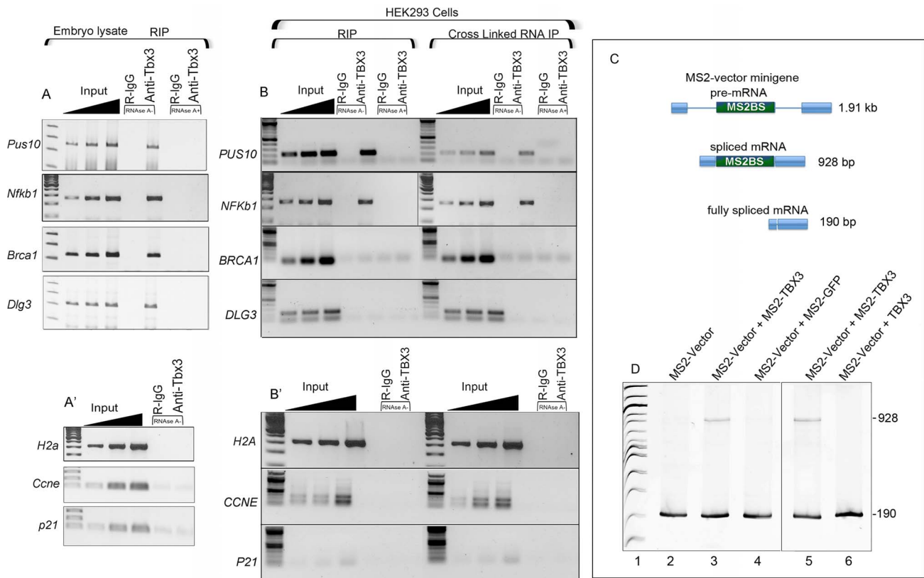
Figure 5. Endogenous Tbx3/TBX3 associates with specific mRNAs in mouse embryonic tissues and HEK293 cells. A, A') RNA-IP with anti-Tbx3 on embryo lysates in the presence or absence of RNaseA followed by RT-PCR for transcript detection. Tbx3 binds Pus10 , NfkB1 , Brca1 and Dlg3 mRNAs. A') H2a, Ccne and p21 are negative controls for the positive interactions seen in panel A, as Tbx3 does not bind/RIP these mRNAs. B, B') RIP and cross-linked RNA-IP (CLIP) of HEK293 lysates followed by RT-PCR. Endogenous TBX3 binds the PUS10 and NFKB1 mRNAs but not BRCA1 , DLG3 (B) or negative controls (B'). C) Schematic of splicing products from a novel splicing reporter containing multimeric MS2 binding sites in exon 2 of the pRHCglo minigene (MS2-vector); the unspliced pre-mRNA (1.91 kb), partially spliced (928 bp), and fully spliced (190 bp) products are shown. D) RT-PCR analysis to detect splicing products from the MS2 reporter RNA in HEK293 cells. In the presence of MS2-TBX3, a partially spliced mRNA is present consisting of exons 1–3, but no introns (927 bp, lanes 3, 5). MS2-GFP (lane 4) and wild type TBX3 (lane 6) have no effect. doi:10.1371/journal.pgen.1004247.g005
