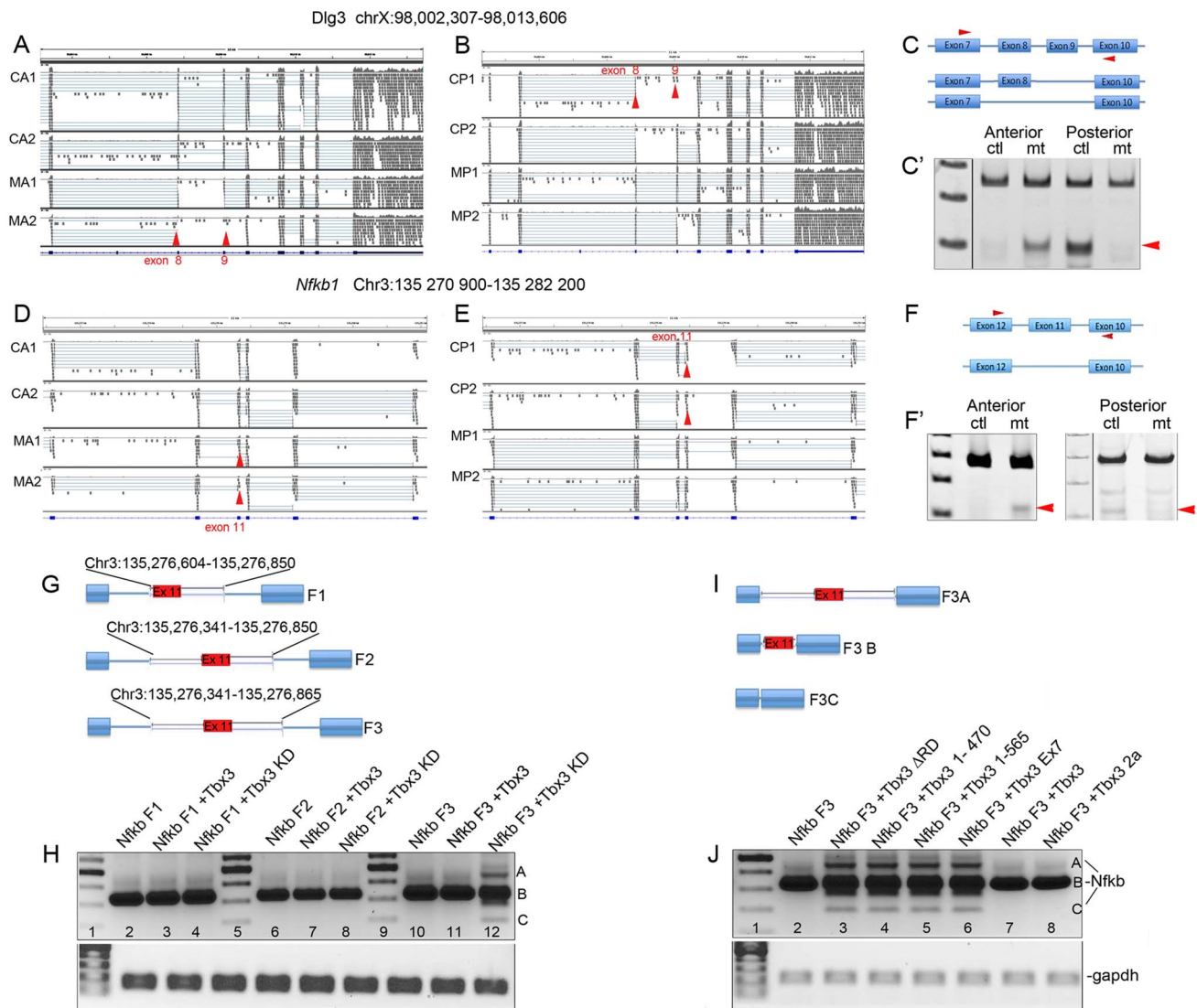
Figure 4. Tbx3 regulates alternative splicing in vivo . A, B, D, E) Screen shots from the Integrated Genome Viewer (IGV) comparing RNA-Seq reads obtained from wild type/control anterior (CA1, CA2) or posterior (CP1, CP2) limb bud mRNA libraries with those from Tbx3;Prx1Cre mutants after conditional ablation of Tbx3 in anterior or posterior limb bud mesenchyme (MA1, MA2 or MP1, MP2, respectively). Red arrowheads indicate positions of exons that are differentially spliced in a Tbx3-dependent manner. A) Loss of Tbx3 causes exclusion of Dlg3 exons 8 and 9 in the mutant anterior compartment (MA1, MA2 red arrowheads). B) Loss of Tbx3 causes inclusion of Dlg3 exons 8 and 9 in the mutant posterior compartment (MP1, MP2 red arrowheads). C) Schematic of splice variants and location of PCR primers used to detect different Dlg3 isoforms by RT-PCR assay of control versus Tbx3 mutant mRNAs (C', Anterior and Posterior compartments, ctl, control; mt, mutant). D) Loss of Tbx3 causes exclusion of Nfkb1 exon 11 in the mutant anterior compartment (MA1, MA2 red arrowheads). E) Loss of Tbx3 causes inclusion of Nfkb1 exon 11 in the mutant posterior compartment (MP1, MP2 red arrowheads). F) Schematic of splice variants and location of PCR primers used to detect different Nfkb1 isoforms by RT-PCR assay of control versus Tbx3 mutant mRNAs (F', Anterior and Posterior compartments, ctl, control; mt, mutant). G) Schematic of Nfkb1 exon 11 minigenes in which exon 2 of pRHCglo was replaced by different Nfkb1 genomic fragments (F1, F2, F3). H) Splicing products assayed by RT-PCR from the Nfkb1 minigenes containing fragments F1, F2 or F3 in the presence of Tbx3 or after knockdown (KD). Only F3 confers differential splicing (lane 12). I) Schematic of splice variants obtained in vivo (sequence confirmed) in response to TBX3 knockdown. J) Splicing products assayed by RT-PCR from the Nfkb1 F3 minigene in the presence of Tbx3 different Tbx3 mutant proteins. C-terminal mutants (lanes 3–6) result in alternate splicing similar to Tbx3 knockdown. doi:10.1371/journal.pgen.1004247.g004
