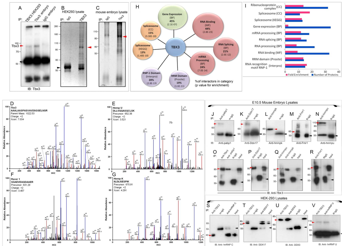
Figure 1. Splicing factors and RNA BPs are over-represented in the Tbx3 interactome identified by MS and are validated co-immunoprecipitation. A) Immunoblot (IB) detecting endogenous TBX3/Tbx3 protein immunoprecipitated (IP) from HEK293 and mouse embryo lysates, respectively. black arrowhead: IgG. B, C) Representative, Coomassie (B, 4–12% gradient) and Oriole stained (C, 10%) SDS-PAGE gels of anti-Tbx3 or negative control IgG IP'd complexes subsequently analyzed by MS. Red arrowheads, TBX3/Tbx3. D–G) Representative mass spectra for identification of Tbx3 (D) and interacting proteins: Hnrnp U (E), Raver 1 (F), Hnrnp K (G). Diagnostic b- and y-series ions are shown in red and blue. H) Gene ontology (GO) analysis identified predominant molecular functions and biological processes of Tbx3 interacting proteins. Diagram shows percent interacting proteins annotated with each GO term (molecular function, MF; biological process, BP; cellular component, CC; functional domain (Interpro and Prosite) and molecular pathway (KEGG). I) Bar graph of number of proteins and fold enrichment per category. J–V) Mouse embryo and HEK293 lysates were immunoprecipitated with the antibody listed at the top of the panels (IP) and the antibodies used to probe the immunoblot (IB) below. J–N) Immunoprecipitation of endogenous: pabp1, Ddx17, hnrnp k, Fmr1, hnrnp u from e10.5 mouse embryo lysates. red arrowheads: interacting protein; black arrowheads: IgG O–R) Endogenous Tbx3 colIPs with pabp1 (O), Ddx17 (P), hnrnp k and hnrnp u (Q), Fmr1 (R) in e10.5 mouse embryos. S–V) Endogenous TBX3 colIPs with hnRNP C (S), DDX17 (T), DDX3 (U) and hnRNP U (V) in HEK293 cells. Red arrowheads: interacting protein; black arrowheads: IgG. doi:10.1371/journal.pgen.1004247.g001
