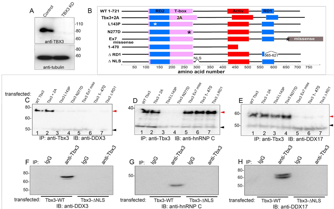
Figure 2. Different Tbx3 protein domains are required for protein-protein interactions. Stable retroviral mediated knockdown of endogenous TBX3 in HEK293 cells followed by transfection of wild type and Tbx3 mutant proteins as diagrammed. Lysate IPs were assayed by IB with antibodies noted at bottom of panels. A) Immunoblot of control versus TBX3 shRNA (KD) lysates. B) Schematic of Tbx3 mutant proteins. Confirmation of expression and successful IP of overexpressed Tbx3 proteins is presented in Figure S2. C–E) Interactions of mutant Tbx3 proteins with DDX3, hnRNP C, and DDX17 tested by IP and western blotting. F–H) Tbx3 NLS is required for Tbx3 interactions with DDX3, DDX17 and hnRNP C. red arrowheads: interacting proteins; black arrowheads: IgG. doi:10.1371/journal.pgen.1004247.g002
