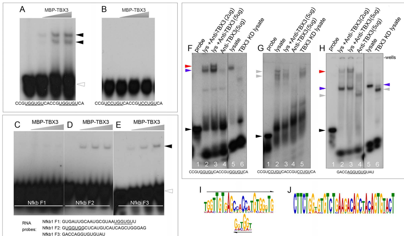
Figure 7. TBX3 binds TBE-containing RNAs directly. A–E) EMSA assays of purified, MBP-conjugated Tbx3 with radiolabeled RNA probes whose sequences are listed at bottom of panels. C–E) RNA probes derived from Nfkb1 intronic fragments (F1–F3). Black arrowheads: probe/protein complex; clear arrowheads: unbound probe. F–H) Shift and supershift RNA EMSA assays of endogenous TBX3; radiolabeled probe sequences are listed below panels. Probes were incubated +/- HEK293 lysate, +/- anti-TBX3 antibody, +/- TBX3 knockdown. F) RNA probe containing GGUGU motifs. Probe/protein complex (lane 5) supershifts with anti-TBX3 antibody (lanes 2, 3) and disappears with TBX3 knockdown (lane 6). TBX3+RNA complexes are indicated by blue arrowheads, anti-Tbx3 antibody supershifted TBX3+RNA complexes are indicated by red arrowheads and unbound probe by black arrowheads. Gray arrowhead indicates probe-protein complexes detected in the absence of TBX3 (lane 6). G) Mutation of the GGUGU to CCUGU results in formation of probe/protein complexes (lane 2) does not supershift with anti-TBX3 antibody (lane 3) and unaffected by TBX3 knockdown (lane 5). H) RNA probe containing AGGUGUG consensus TBE motif from Nfkb1 Fragment 3. Probe/protein complex (lanes 2, 3, 5, blue arrowhead) supershifts with anti-TBX3 antibody (lanes 2, 3, red arrowheads) and decreases with TBX3 knockdown (lane 6). Gray arrowhead indicates probe-protein complexes detected in the absence of TBX3 (lane 6). Probe incubated with no lysate (F–H, lanes 1) or anti-TBX3 antibody alone (F–H, lanes 4) are additional negative controls. IgG negative control EMSAs are shown in Figure S5 G, H, I, J). Significantly over-represented sequence motifs identified by MEME on genomic regions flanking statistically significant AS events contain the 5'GGTG T-box core binding element. doi:10.1371/journal.pgen.1004247.g007
