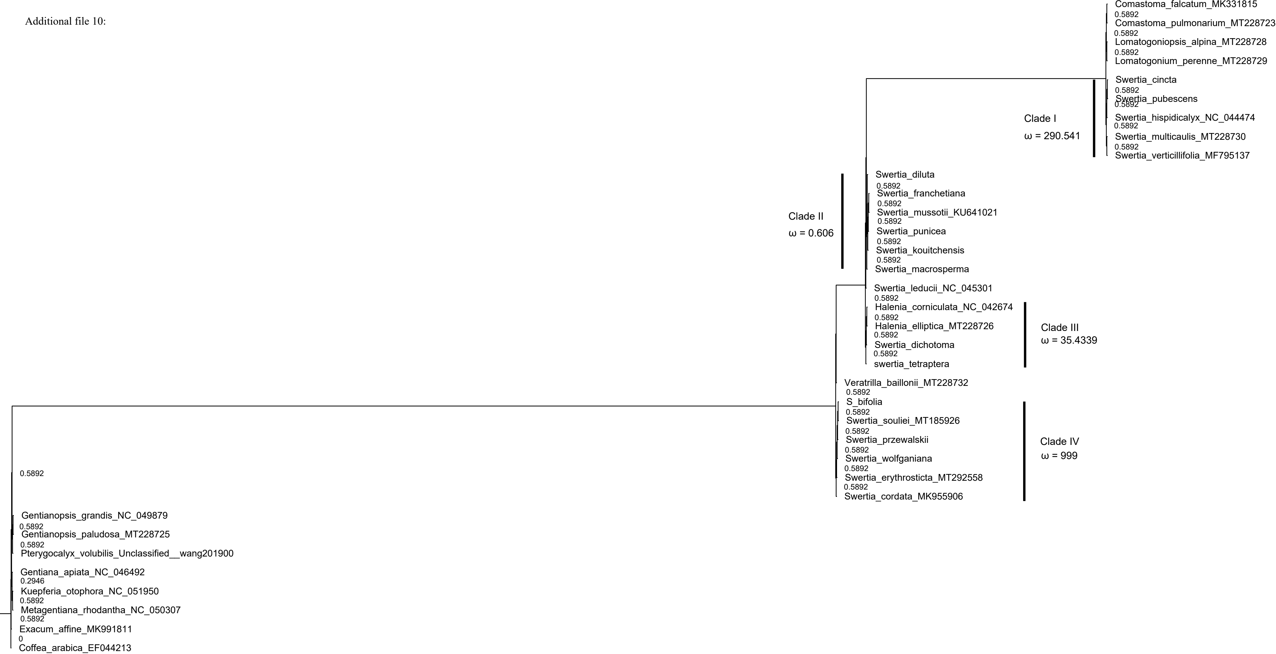
Supplementary Figure S2 The \omega ratio of cemA along the phylogenetic tree of Gentianaceae
