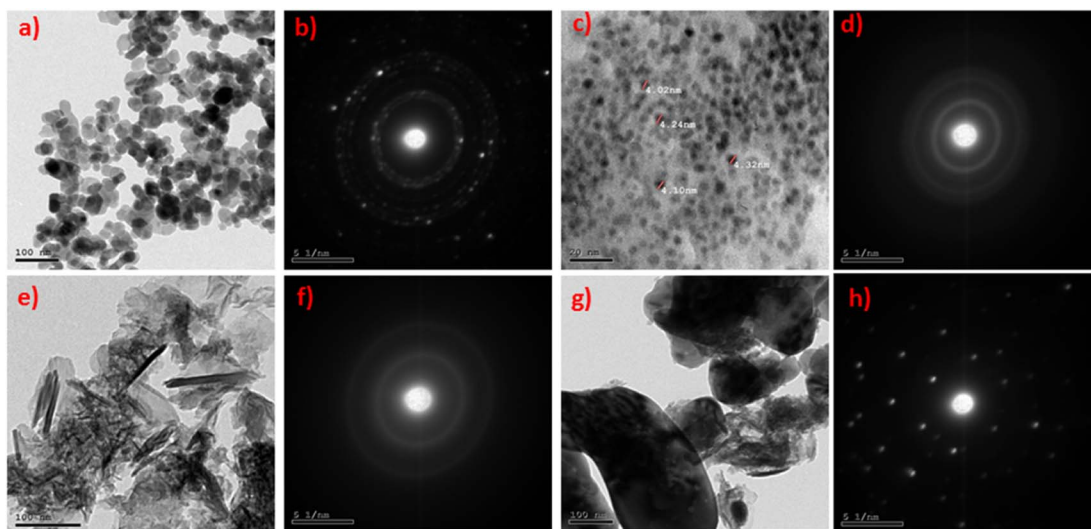
Fig. 5 The HR-TEM images and the corresponding SAED patterns of (a and b) ZnO NPs, (c and d) CdSQDs, (e and f) ZnCr-LDO nanosheet, and (g and h) CdSQDs@ZnCr-LDO/ZnO ternary nanocomposite.
