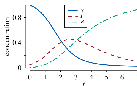
Figure 1. SDS interpretation of the SIR curves. The S_t curve is the survival function for time to infection: S_t = P(T_I > t) where T_I is the time at which an individual moves from the susceptible to the infected compartment. The R_t curve, upon multiplication with \mathcal{R}_0 , gives the corresponding cumulative hazard. Finally, the convolution of the infection time T_I and the infectious time T_R (time spent in the infected compartment) is given by the I_t curve, after adjustment for the initial infecteds. Parameter values: \beta = 2 , \gamma = 0.5 with initial condition S_0 = 1 , I_0 = 0.05 and R_0 = 0 . (Online version in colour.)
