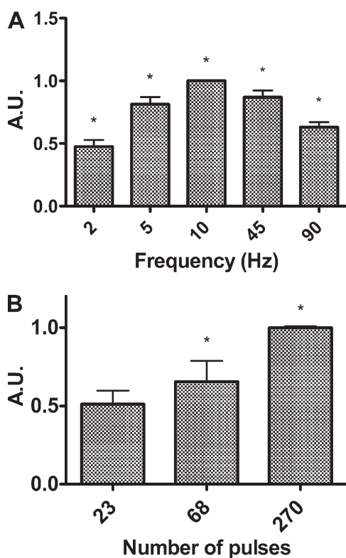
Figure 3. The slow Ca^{2+} signal is dependent on frequency and duration of the electrical stimulus. (A) Individual isolated FDB fibers were stimulated with 270 pulses at 2, 5, and 10 Hz or at 10, 45, and 90 Hz (and in the inverted sequence 10, 5, and 2 Hz and 90, 45, 10 Hz). The magnitude of the slow Ca^{2+} signal was measured as the area under the curve in the post-tetanic region. The values are arbitrary units normalized against the area corresponding to 10 Hz. The graph shows the mean area of different fibers stimulated in both sequences of stimulation frequency. We observe a bell-shaped curve, depending on frequency, with a maximum at 10 Hz. Differences between each pair of frequencies, for each frequency series (i.e., 2 vs. 5, 2 vs. 10, and 5 vs. 10; 10 vs. 45, 10 vs. 90, and 45 vs. 90), are statistically significant (*, P < 0.05 ). (B) The magnitude of slow signal was dependent on the duration of electrical stimuli. The graph shows the mean values for different fibers stimulated at 45 Hz with 23, 68, and 270 pulses. The area values are arbitrary units normalized against signal corresponding to 270 pulses. We observe that the signal magnitude increases with the increase in the stimulus duration. (*, P < 0.05 )
