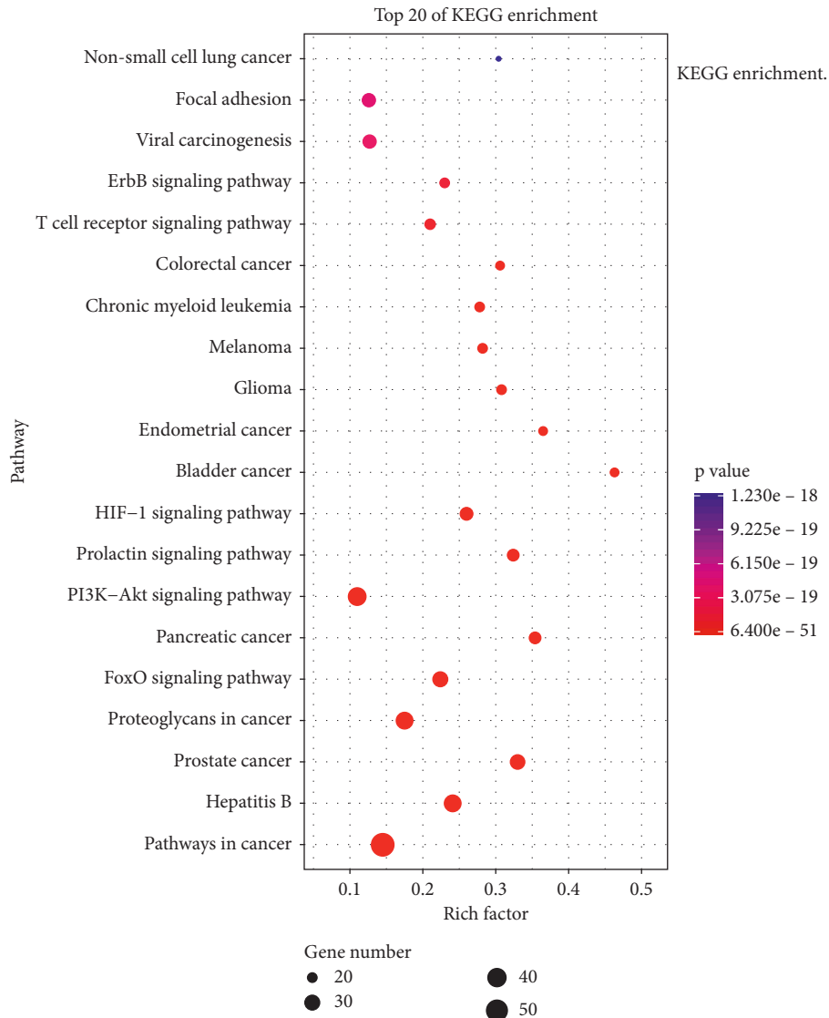
FIGURE 7: KEGG enrichment.
