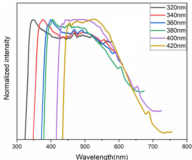
Fig. 9 Emission spectra of 4-BAPC with different wavelengths excitation at room temperature.
