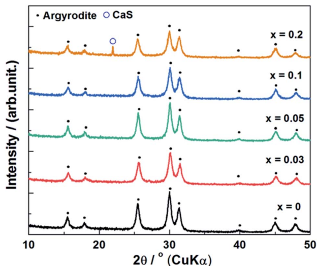
Fig. 1 X-ray diffraction patterns of (1-x)\text{Li}_6\text{PS}_5\text{Cl}-x\text{CaS} ( 0 \leq x \leq 0.2 ) synthesized by ball milling method.
