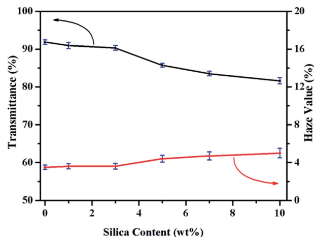
Fig. 9 Effect of \text{SiO}_2 - g -PLA on the transmittance and haze value of PLA.
