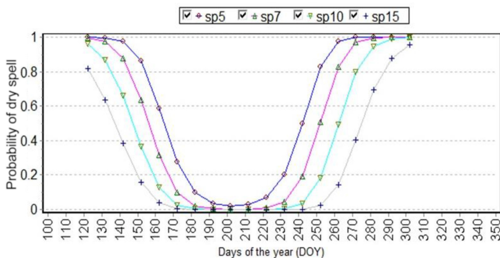
Figure 3. Unconditional dry spells length for Woreta station over the period 1986–2017.
