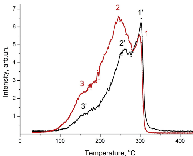
Fig. 2. Hydrogen isotopes release: H ( 1'-3' ) and D (1–3) from the closed loop of Pd at the linear heating mode (heating rate = 1\text{ }^\circ\text{C}\cdot\text{s}^{-1} ) by a quartz coaxial furnace ( j = (30-70)\text{ A cm}^{-2} ) in a quartz vacuum cell: 1, 1' peaks are the thermal stimulation contribution: T_{max1}(D_2) , T_{max1}'(H_2) = 300\text{ }^\circ\text{C} ; 2, 2' peaks are the electromagnetic field contribution: T_{max2}(D_2) = 246\text{ }^\circ\text{C} , T_{max2}'(H_2) = 262\text{ }^\circ\text{C} ; 3, 3' peaks are the induced electric current contribution: T_{max3}(D_2) , T_{max3}'(H_2) = 16\text{ }^\circ\text{C} . Electrolytic saturation of Pd: D_2SO_4 (0.5 M), t = 90\text{ min} , I = 100\text{ mA} , 02.15.2018.
