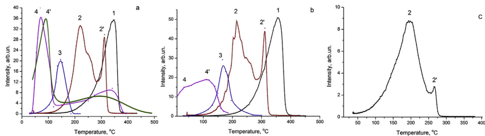
Fig. 1. The hydrogen isotopes release ((a) – H_2 , (b) – (D_2) ) from Pd at the linear heating: in stainless steel vacuum cell T_{max}(H_2) = 355\text{ }^\circ\text{C} , T_{max}(D_2) = 360\text{ }^\circ\text{C} (curves 1 a, 6); in quartz vacuum cell T_{max}(H_2) = 220\text{ }^\circ\text{C} (peak 2a), T_{max}(H_2) = 312\text{ }^\circ\text{C} (peak 2'a), T_{max}(D_2) = 217\text{ }^\circ\text{C} (peak 2b), T_{max}(D_2) = 311\text{ }^\circ\text{C} (peak 2'b); heating by AC: T_{max}(H_2) = 150\text{ }^\circ\text{C} , T_{max}(D_2) = 165\text{ }^\circ\text{C} (curves 3 a,6); radiation-stimulated hydrogen release (curves 4 a,b); analytical approximation of the experimental curve 4a (кривая 4a').
