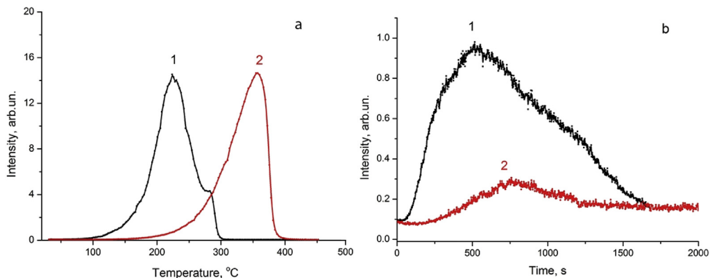
Fig. 3. Deuterium release from palladium at linear heating: (a) – heating rate is 1\text{ }^{\circ}\text{C s}^{-1} with simultaneous irradiation of the palladium surface with UV (curve 1) and without UV irradiation (curve 2); (b) – heating rate is 0.1\text{ }^{\circ}\text{C/s} , sample temperature from 25 to 65\text{ }^{\circ}\text{C} ( 0\text{ t}^{\circ} 650\text{ s} ) with simultaneous irradiation of the palladium surface with UV (1b) and without UV (2b); (1b) – t_{\text{max UV}} = 560\text{ s} , (2b) t_{\text{max T}} = 770\text{ sec} ; sample size: 0.05 \times 3 \times 25\text{ mm} . Electrolytic saturation of Pd in \text{D}_2\text{SO}_4 (1,0 M) + in \text{D}_2\text{O} , t = 2\text{ h} , i = 70\text{ mA cm}^{-2} .
