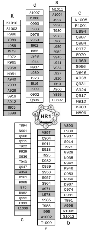
Figure 1: Schematic representation of SARS-CoV (strain TOR2) spike protein, sequence similarities between SARS-CoV and HIV-1 N-peptides and C-peptides, and helical wheels of HR1 and HR2
