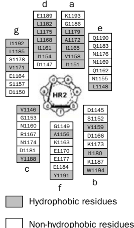
Figure 1: Schematic representation of SARS-CoV (strain TOR2) spike protein, sequence similarities between SARS-CoV and HIV-1 N-peptides and C-peptides, and helical wheels of HR1 and HR2
