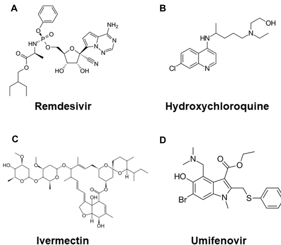
Figure 1 The chemical structures of the COVID-19 antivirals: (A) remdesivir; (B) hydroxychloroquine; (C) ivermectin; (D) umifenovir. Structures are courtesy of Wikipedia.
