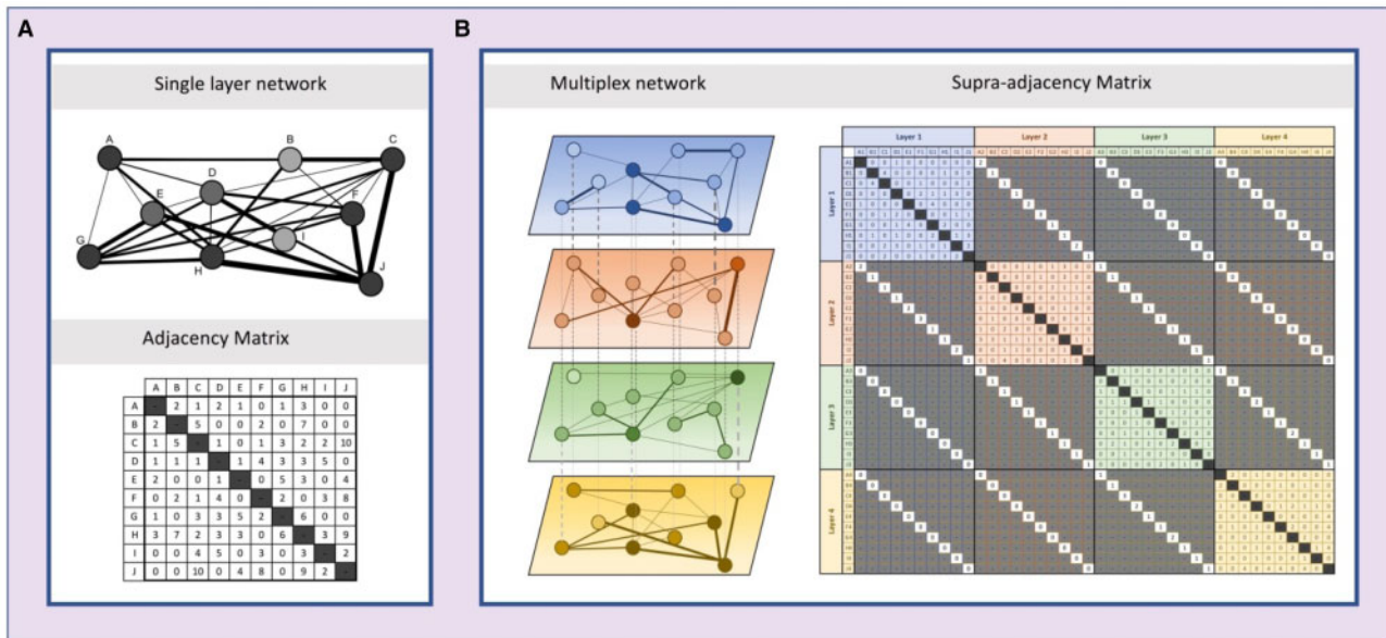
Figure 1. Single and multilayer networks and their matrices. A single layer network (A) is comprised of nodes (labeled A–J) connected by undirected edges whose weights are indicated by the thickness of the lines. If there are multiple types of connections that form edges, they could instead be separated into multiple distinct network layers as a multiplex network (B). Here, there is a copy or “node-tuple” of each A–J node on each layer, which are connected to each other across layers.
