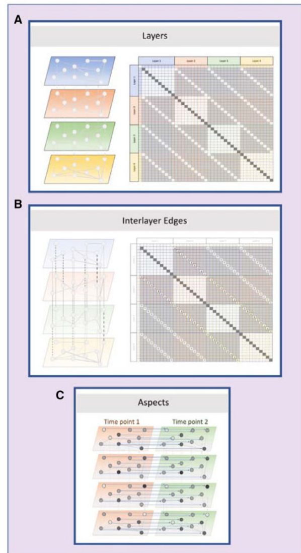
Figure 3. Unique multilayer network characteristics. There are parts of a multilayer network and their corresponding locations on a supra-adjacency matrix that do not exist on single layer networks or their adjacency matrices. In the same way that individuals are organized across columns and rows in an adjacency matrix, layers (colored rectangles in panel A) are organized as sets of columns and rows in the corresponding supra-adjacency matrix (colored sections in panel A). This structure creates cells that correspond to all combinations of all node-tuples. In a multiplex network where interlayer edges only connect to node-tuples of the same node, interlayer edges (dotted lines connecting nodes across layers in panel B) only exist across the diagonals of the matrices that represent connections across different layers (bold values in panel B). In this network, node-tuples are only connected on networks that are next to each other, so some of these values are 0 for layers that are not adjacent. If node-tuples were connected to their counterparts on all layers, all of these diagonals would have non-zero values. If the network is not a multiplex network and allowed node-tuples to be connected to node-tuples of different individuals across layers, cells other than the diagonals in these interlayer matrices could have values. If interlayer edges are directed, these values would not be symmetrical across the diagonal of the whole supra-adjacency matrix, as they are in panel B. Finally, multilayer networks can be represented as stacks of different layers (i.e., aspects, orange and green stack of layers in panel C), and nodes can be connected across aspects. While the supra-adjacency matrix is not shown here, it would increase in scale in a similar way from the jump from single to multiple layers, but to include copies of all of these parts for multiple aspects that themselves could be connected.
