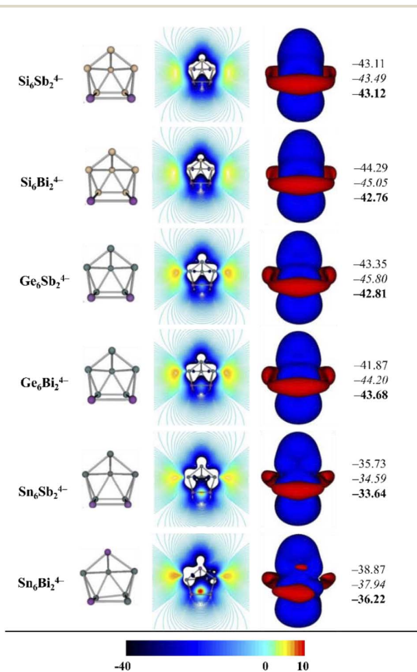
Fig. 4 Isosurface and contour plot for B_z^{\text{ind}} and the external field ( \text{NICS}_{zz} ). The isosurface value is set to \pm 3.0 ppm. Blue: long range shielding regions; red: deshielding regions. B_z^{\text{ind}} values at the cage center are reported at the PBE0/def2-TZVP, PBE0-ZORA/TZ2P (italic) and PBE0-SO/TZ2P (bold) levels.
