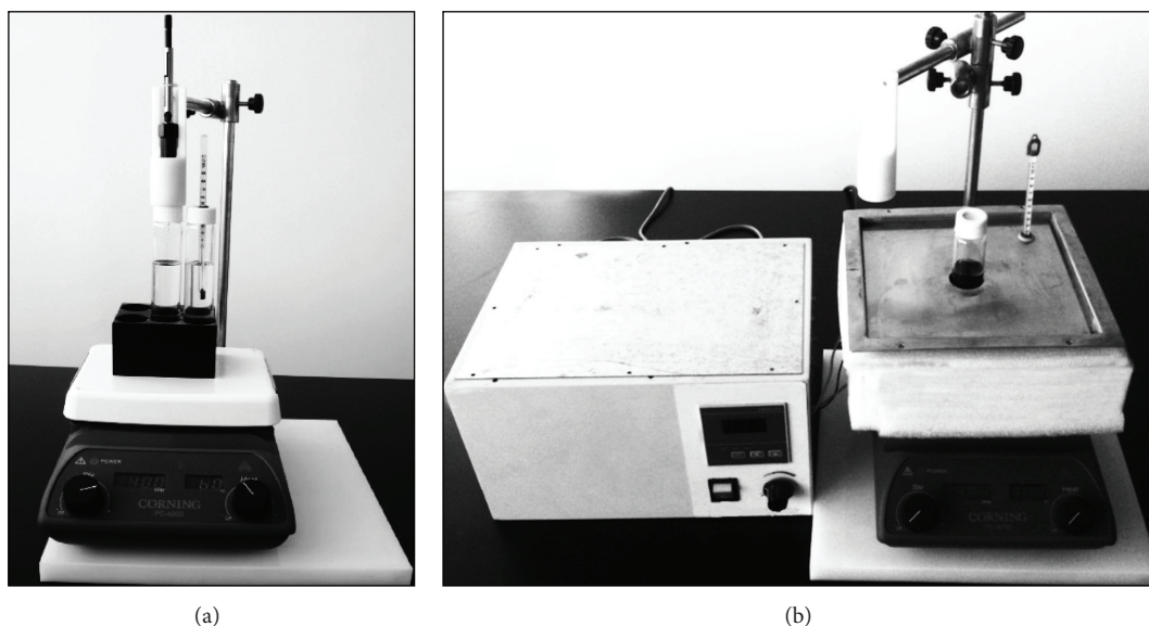
FIGURE 1: (a) The original magnetic stirrer from CORNING and (b) modified one.
