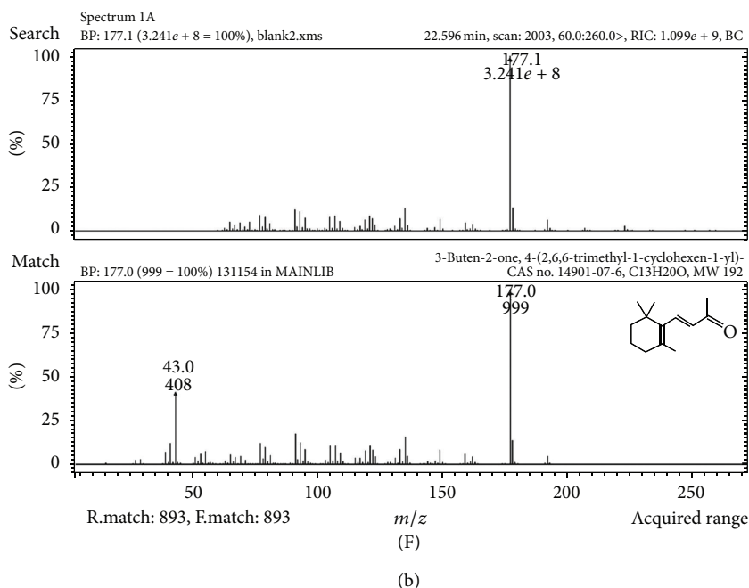
FIGURE 3: (a) MS-chromatogram of water sample (total ion current of the MS in the select ion mode) and (b) mass spectra of the six target compounds. Shown are (A) DMTS, (B) IBMP, (C) 2-MIB, (D) \beta -cyclocitral, (E) GSM, and (F) \beta -ionone for both (a) and (b).
