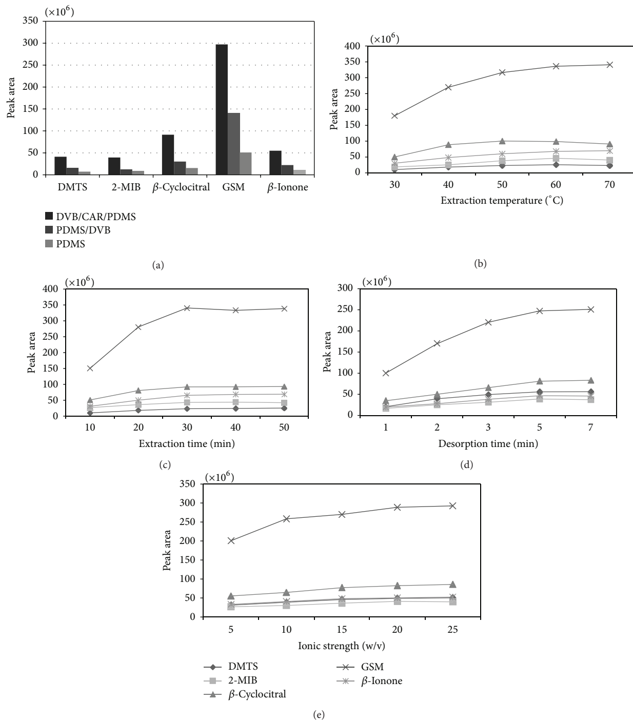
FIGURE 2: The effect of (a) fiber, (b) extraction temperature, (c) extraction time, (d) desorption time, and (e) ionic strength on the HS-SPME/GC-MS of five target compounds, and 100 ng L -1 of mixed standard solutions was analyzed by (a) fiber exposition at 60 °C, 30 min, for 25% (w/v) ionic strength, (b) fiber exposition at 25% (w/v) ionic strength for 30 min, (c) fiber exposition at 60 °C for 25% (w/v) ionic strength, and (d) and (e) at 60 °C for 30 min.
