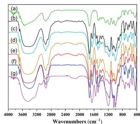
Fig. 2 FTIR spectra of nanocomposite hydrogels. A-HNC (a), B-DHNC3 (b), B-DHNC5 (c), B-DHNC7 (d), C-DHNC (e), D-DHNC (f), and E-DNC (g).
