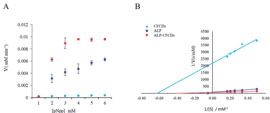
Fig. 2 ALP enzyme kinetics upon CFCD coenzyme addition. (A) The plot of the initial reaction rate ( V ) versus the pNPP substrate ( S ) concentration at 25\text{ }^\circ\text{C} and pH 7. (B) The plot of 1/V versus 1/[S] .
