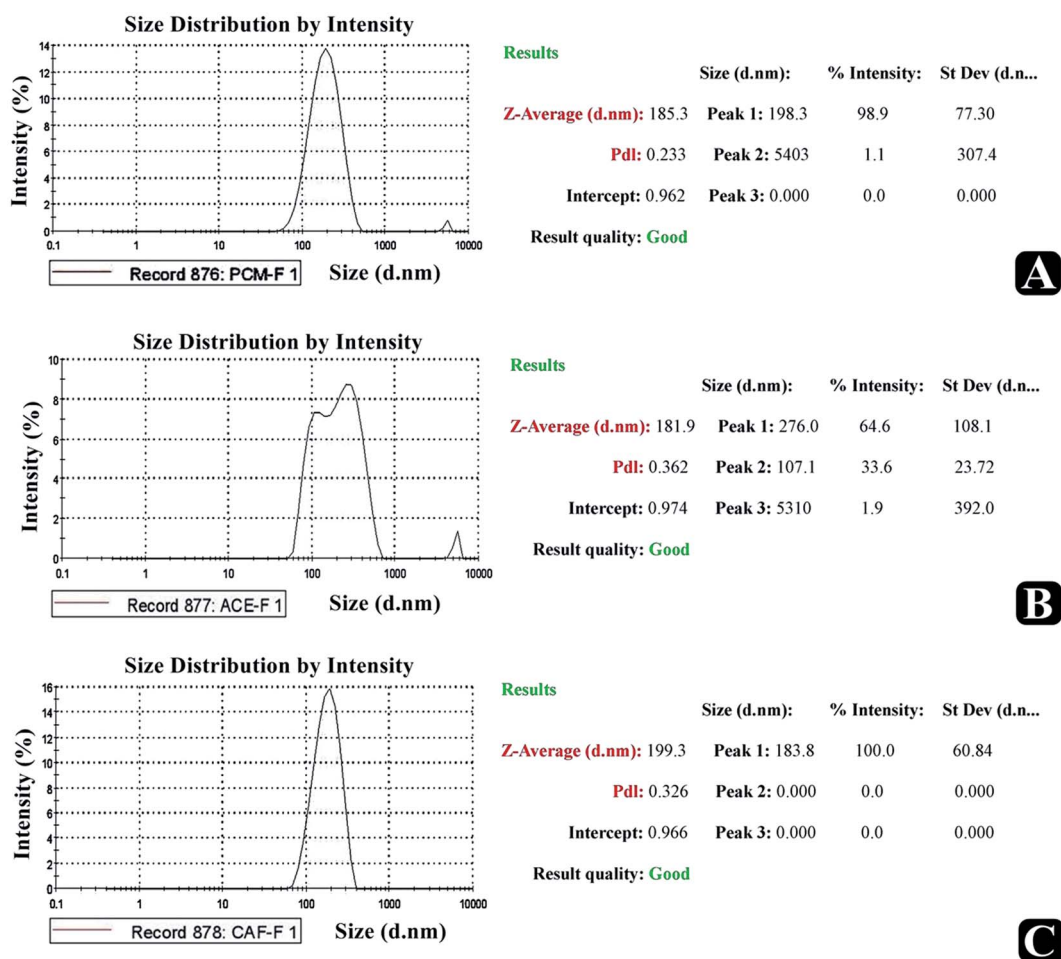
Fig. 6 Particle size analysis report.
