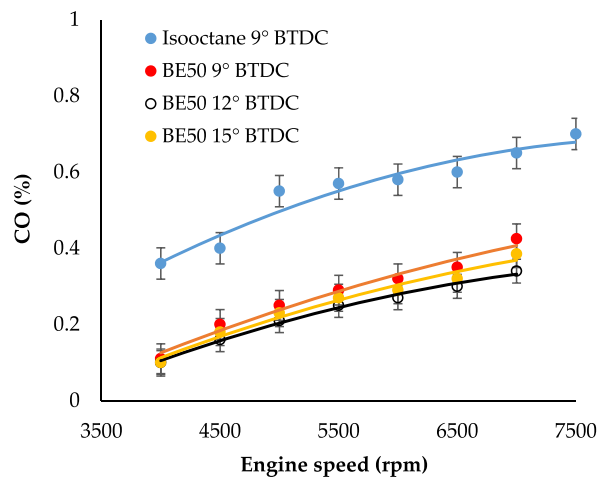
Fig. 8. CO emission of SI engine at various ignition timings.
