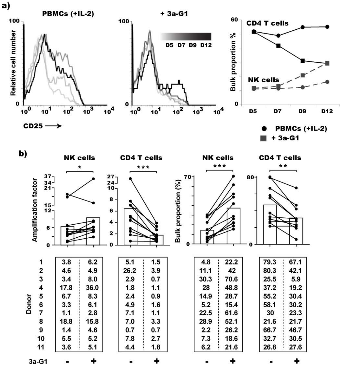
Figure 2 3a-G1 treated PBMCs show progressive enrichment in NK cells at CD4 + T cell expense during the second week of culture. a) CD25 expression gated on CD4 + T cells (left graphs) and NK cell versus CD4 + T cell proportion at days 5, 7, 9 and 12 of culture (right graph). b) Amplification factor (left) and proportion (right) of NK and CD4 + T cell populations among PBMCs from eleven different donors after 12 to 14 days treatment with 3a-G1 . Histograms indicate the means of the data collected from the eleven donors (Wilcoxon signed rank t test, *: P ≤ 0.05, **: P ≤ 0.01, ***: P ≤ 0.001).
