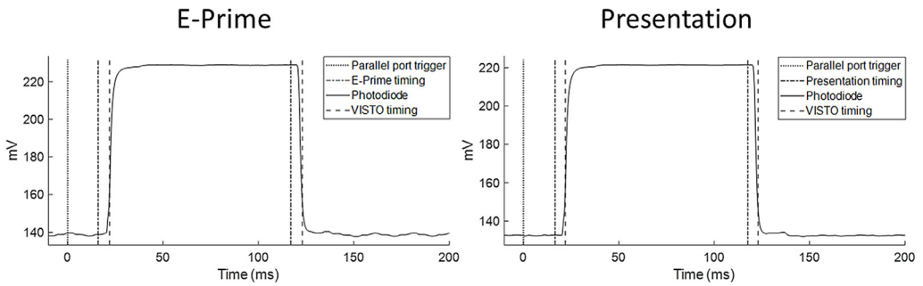
Fig. 9. Comparison of event timings by VISTO and E-Prime (left) and Presentation (right). The parallel port input coming from the presentation PC is shown as a dotted vertical line. The veridical stimulus signal (solid line: screen luminance recorded through a second photodiode acquired with a BIOPAC system) is plotted together with the event markers indicated by presentation software (dashed-dotted lines) and by VISTO (dashed lines).
