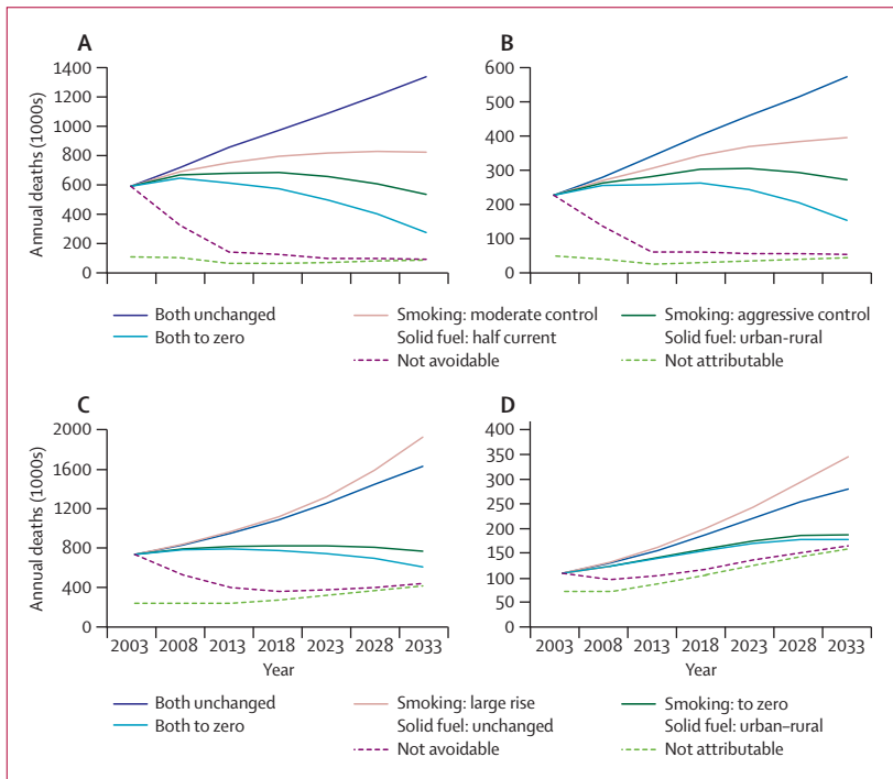
Figure 2: Annual mortality in men from COPD (A) and lung cancer (B) and in women from COPD (C) and lung cancer (D) under combined scenarios of smoking and solid fuel use. Not avoidable deaths are those if risk-factor exposures were reduced to zero in 2003. See webfigures 4 and 5 for separate results for smoking and solid fuel use.
