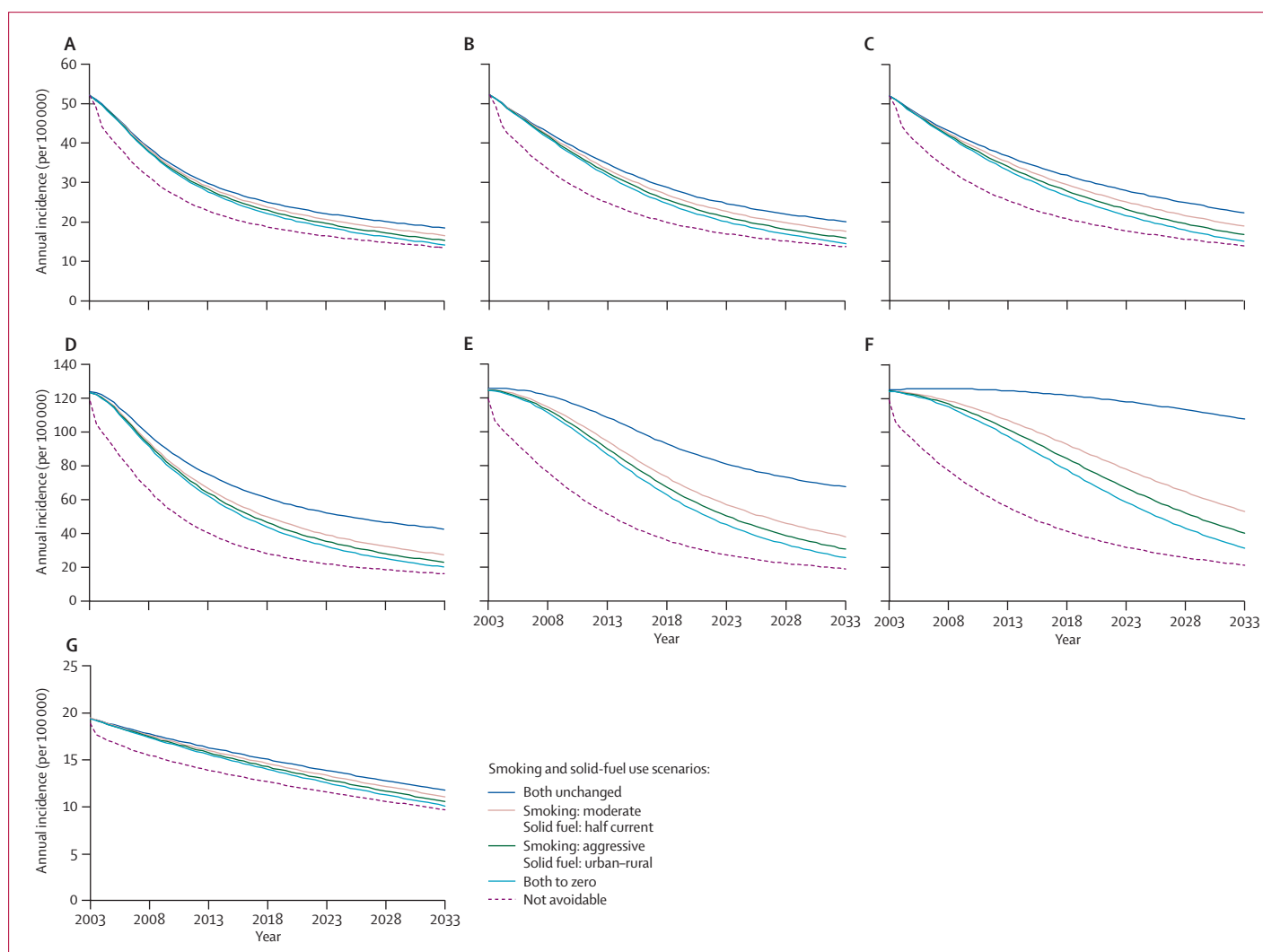
Figure 4: Annual incidence of infectious tuberculosis under combined effects of smoking and indoor air pollution scenarios by municipality and DOTS effectiveness
