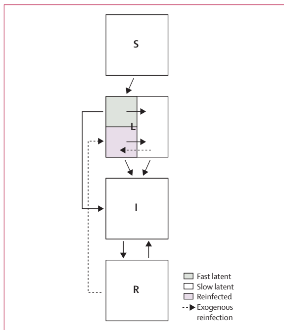
Figure 1: Compartmental susceptible-latent-infectious-recovered (SLIR) model of tuberculosis infection
