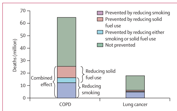
Figure 3: Sum of annual deaths 2003–33 for both sexes if exposure for both sexes to smoking and solid fuel use are reduced to zero by 2033
