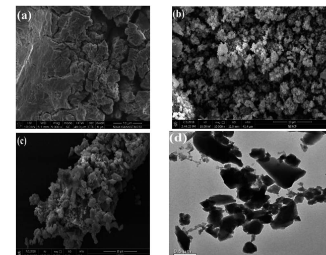
Fig. 4 SEM images of pristine PMA (a), Fe-BTC (b), PMA/Fe-BTC (c) catalyst and TEM images of the PMA/Fe-BTC (d) catalyst.
