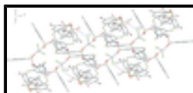
Fig. 3. A view of the one-dimensional chain of the dimers approximately along the b axis. Some hydrogen atoms are omitted for clarity. [Symmetry codes: (i) -x + 1, -y + 2, -z ; (ii) x - 1, y, z ; (iv) -x, -y + 2, -z ].
