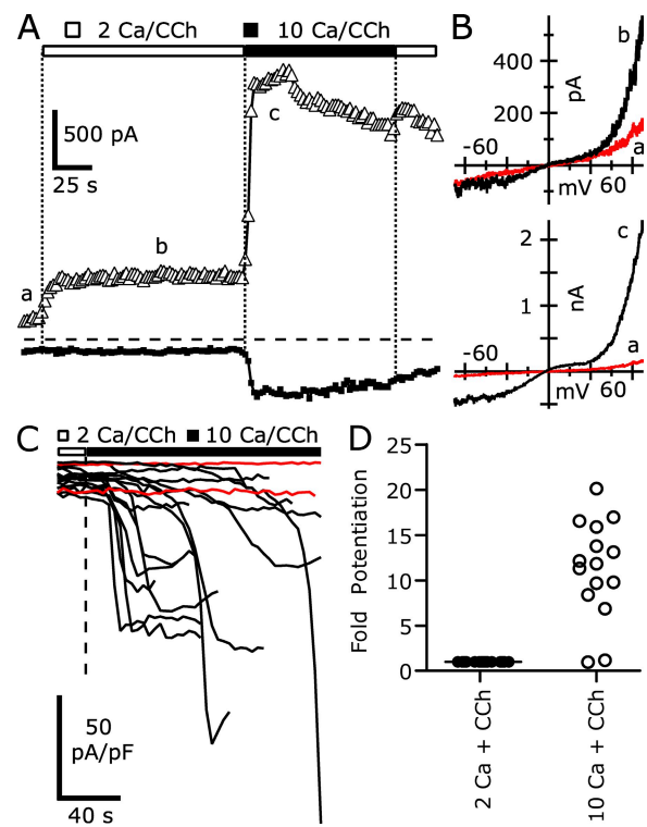
Figure 4. The application of 10 mM of extracellular Ca 2+ rapidly induces large-amplitude TRPC5 currents in TRPC5 and M1R cotransfected HEK cells. (A) The average TRPC5-mediated currents at +100 mV (triangles) and at -40 mV (squares). Open and black bars indicate the timing of the addition of external solution. (B) I-V curves taken from ramps applied at the times shown by the lowercase letters in A. Currents before (top) and after (bottom) potentiation are shown. (C) The average current densities at -40 mV of 15 cells in response to 10 Ca external; before calcium increase, the bath contained 2 Ca external solution + 100 μM CCh. Cells that were potentiated are shown in black, and unpotentiated cells are shown in red. (D) Potentiation of current at -40 mV in 10 Ca 2+ external (right) relative to 2 Ca external (left) in the internal solution (in mM): 150 Cs-Asp, 2 MgCl 2 , 0.36 CaCl 2 , 1 EGTA, 4 MgATP, 0.3 NaGTP, and 10 HEPES, pH 7.20 with CsOH (100 nM calculated free [Ca 2+ ]). External solution: 2 or 10 Ca external, both with 1 mM MgCl 2 .
