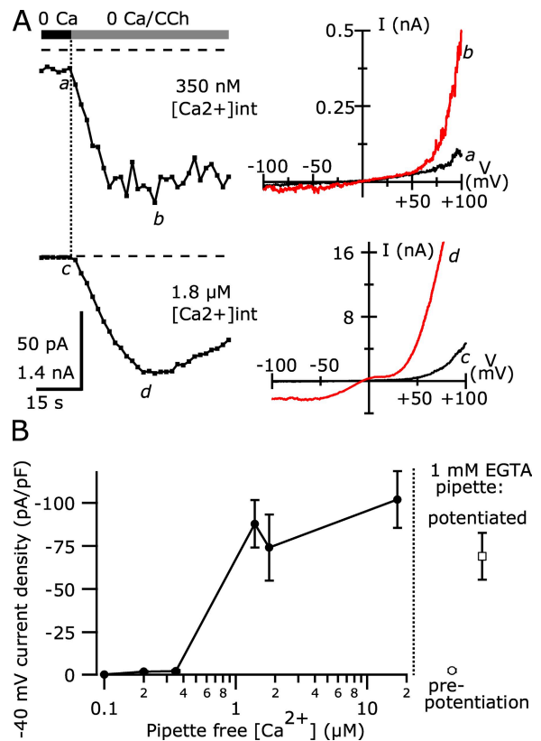
Figure 6. Internal free [Ca^{2+}] > 1 \mu M dramatically increases TRPC5 current density. (A; Left) The average CCh-activated current at -40 mV in a TRPC5/M1R-expressing cell recorded with an internal solution containing \sim 350 nM of calculated free [Ca^{2+}] (top) and in a different cell recorded with an internal solution with \sim 1.8 \mu M of calculated free [Ca^{2+}] (bottom). The currents recorded with 350 nM of calculated free [Ca^{2+}] are shown on an expanded current scale. (Right) I-V curves elicited by ramp voltage stimuli before the application of 100 \mu M CCh ( a ) and during the peak of the response ( b ). The external solution was nominally Ca free. The currents recorded with 350 nM of calculated free internal [Ca^{2+}] were digitally smoothed using a Gaussian filter ( -3 db = 1 kHz; top). (B) The average peak CCh-activated current density at -40 mV from cells recorded with internal solutions with varying calculated free internal [Ca^{2+}] . Also shown are the average current densities at -40 mV of CCh-activated TRPC5 currents in nominally Ca-free external solution before and after potentiation, recorded with 1 mM of EGTA-containing internal solutions. The average current density at -40 mV with 100 nM of calculated free [Ca^{2+}] was -0.40 \pm 0.08 pA/pF ( n = 8 ), with 200 nM it was -2.08 \pm 0.37 pA/pF ( n = 22 ), and with 350 nM it was -2.44 \pm 0.63 pA/pF ( n = 8 ). Higher calculated free [Ca^{2+}] values gave the following: 1.4 \mu M , -87.95 \pm 13.81 pA/pF ( n = 10 ); 1.8 \mu M : -74.13 \pm 19.19 pA/pF ( n = 7 ); and 17 \mu M : -102.03 \pm 16.38 pA/pF ( n = 9 ). Error bars represent \pm SEM; missing error bars are smaller than symbols. Internal solutions with calculated [Ca^{2+}] < 350 nM each contained (in mM): 110 Cs-Asp, 10 CsCl, 2 MgCl 2 , 10 Cs 4 -BAPTA, 4 MgATP, 0.3 Na-GTP, and 10 HEPES, pH 7.20 with CsOH, with 3.1 CaCl 2 for 100 nM [Ca^{2+}] , 4.7 mM CaCl 2 for 200 nM, and 6.0 mM CaCl 2 for 350 nM. Internal solutions with calculated free [Ca^{2+}] > 1 \mu M each contained (in mM): 150 Cs-Asp, 2 MgCl 2 , 4 MgATP, 0.3 NaGTP, and 10 HEPES, pH 7.20 with CsOH, and the following CaCl 2 and HEDTA: 1.11 CaCl 2 and 10 HEDTA for 1.4 \mu M [Ca^{2+}] , 0.43 CaCl 2 and 5 HEDTA for 1.8 \mu M [Ca^{2+}] , and 1.89 CaCl 2 and 5 HEDTA for 17 \mu M [Ca^{2+}] .
