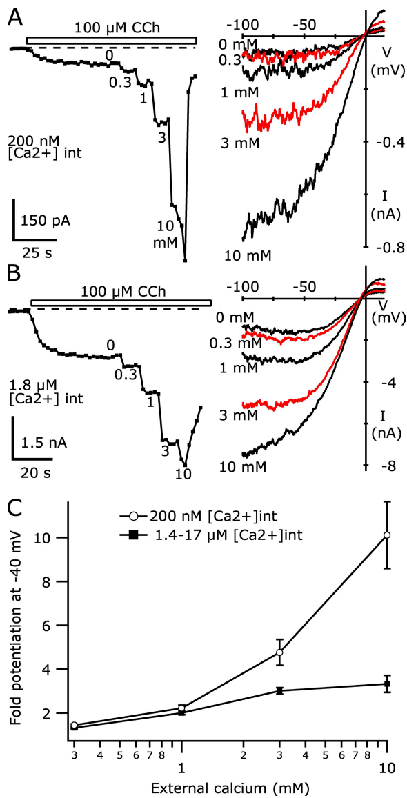
Figure 12. The extent of TRPC5 current potentiation by intracellular \text{Ca}^{2+} affects external \text{Ca}^{2+} current enhancement. (A) The average current at -40 mV recorded in a TRPC5/MIR-expressing HEK cell (left); internal solution with 200 nM of calculated free [\text{Ca}^{2+}] containing (in mM): 110 Cs-Asp, 10 CsCl, 2 \text{MgCl}_2 , 4.7 \text{CaCl}_2 , 10 \text{Cs}_4\text{-BAPTA} , 4 \text{MgATP} , and 0.3 \text{NaGTP} , pH 7.20 with CsOH. The right panels here and in B show the I-V curves from each initial sweep in different [\text{Ca}^{2+}] . Currents recorded in 0.3 and 3 mM of external \text{Ca}^{2+} are shown in red; all others are shown in black. (B) The average current at -40 mV using an internal solution with 1.8 \mu\text{M} of calculated free [\text{Ca}^{2+}] containing (in mM): 150 Cs-Asp, 2 \text{MgCl}_2 , 0.46 \text{CaCl}_2 , 5 HEDTA, 4 \text{MgATP} , and 0.3 \text{NaGTP} , pH 7.20 with CsOH. (C) Potentiation of current at -40 mV relative to that in nominally Ca-free external solution is plotted versus external [\text{Ca}^{2+}] for cells recorded in 200 nM of internal calculated free [\text{Ca}^{2+}] (open circles) or 1.4–17 \mu\text{M} of calculated free [\text{Ca}^{2+}] (filled squares). Potentiation for the 200 nM Ca internal was 1.44 \pm 0.05 -fold for 0.3 Ca, 2.22 \pm 0.14 -fold for 1 Ca, 4.77 \pm 0.59 for 3 Ca, and 10.11 \pm 1.53 for 10 Ca ( n = 6 each); whereas, for the >1.4 \mu\text{M} [\text{Ca}^{2+}] internals it was 1.32 \pm 0.04 -fold, 2.00 \pm 0.08 , 3.09 \pm 0.15 , and 3.33 \pm 0.39 ( n = 10 ; n = 8 for 10 Ca external). External solutions had the following added divalents (in mM):
