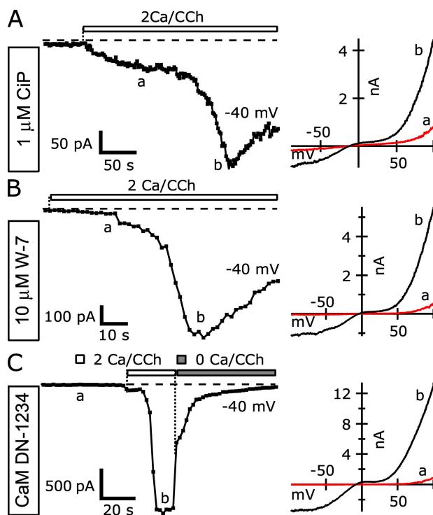
Figure 14. Calmodulin inhibition does not prevent potentiation of TRPC5 by intracellular \text{Ca}^{2+} . (A–C; Left) The average currents at -40 mV (squares) recorded from TRPC5 and MIR cotransfected HEK cells during voltage ramps demonstrate \text{Ca}^{2+} potentiation in the presence of calmodulin inhibitors. (Right) I–V relations corresponding to points at left indicated by the lowercase letters. (A) Internal 1 \mu\text{M} of calmodulin inhibitory peptide ( n = 5 ). (B) Internal 10 \mu\text{M} W-7 ( n = 4 ). (C) Coexpression of a dominant-negative mutant calmodulin (CaM DN-1234) with TRPC5. Internal Solution (in mM): 150 Cs-Asp, 2 \text{MgCl}_2 , 0.36 \text{CaCl}_2 , 1 EGTA, 4 \text{MgATP} , 0.3 \text{NaGTP} , and 10 HEPES, pH 7.20 with CsOH (100 nM of calculated free [\text{Ca}^{2+}] ). External solution: 2 Ca and nominally Ca-free external.
