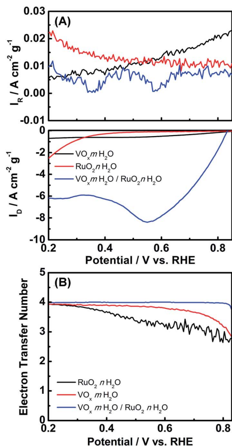
Fig. 4 (A) The RRDE voltammograms and (B) the mean electron transfer number ( n ) of the ORR obtained from the GC disk electrode deposited with (1) \text{VO}_x \cdot m\text{H}_2\text{O}/\text{RuO}_2 \cdot n\text{H}_2\text{O} , (2) \text{VO}_x \cdot m\text{H}_2\text{O} , and (3) \text{RuO}_2 \cdot n\text{H}_2\text{O} in \text{O}_2 -saturated 0.5 M \text{Na}_2\text{SO}_4 with pH = 3 at 5 \text{ mV s}^{-1} and a rotating speed of 900 rpm.
