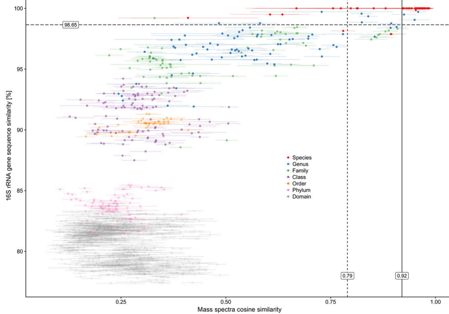
FIGURE 3 | Plot showing pairwise relationship of 16S rRNA gene sequence similarity between two cultures and their mass spectra cosine similarity. Horizontal error bars represent standard deviations of mass spectra cosine similarities calculated for all technical and biological replications ( n = 3 \times 4 = 12 ). The colors of the data points represent the lowest taxonomy rank that is shared between a pair of microorganisms. The taxonomical classification and species assignment by the closest type strain were carried out using the EzCloud Identify Service. Vertical solid line —calculated optimal cosine similarity threshold based on 98.65% 16S rRNA gene similarity; vertical dashed line —calculated optimal cosine similarity threshold based on assigning the closest type strain.
