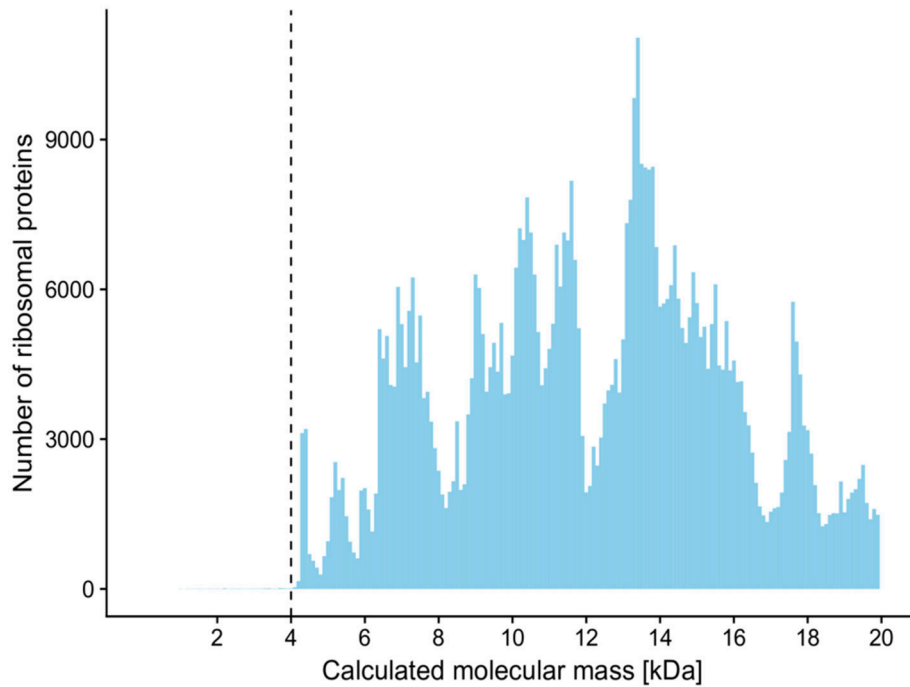
FIGURE 2 | Histogram of calculated molecular masses of bacterial ribosomal proteins. Only 123 (0.01%) proteins out of 761,208 had a molecular mass of less than 4 kDa. Molecular masses were calculated and downloaded from the UniProtKB protein database. The histogram is made up of bins of 100 Da, and only proteins with a mass of less than 20 kDa are shown.
