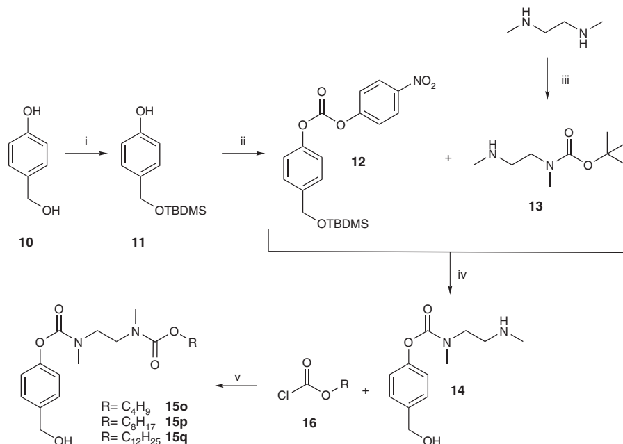
Figure 2 | Reagents and conditions. (i) TBDMSCl, imidazole, \text{CH}_2\text{Cl}_2 , rt, 2 h; (ii) 1 , 4-nitrophenyl chloroformate, triethylamine, \text{CH}_2\text{Cl}_2 , rt, 16 h, 2 , triethylene glycol monomethyl ether, rt, 20 min; (iii) \text{Boc}_2\text{O} , 0^\circ\text{C} -rt, 20 h; (iv) 1 , 4-DMAP, diisopropylethylamine, toluene, rt, 16 h, 2 , TFA/ \text{CH}_2\text{Cl}_2 , rt, 0.5 h; (v) 1 , TMSCl, imidazole, THF, 0^\circ\text{C} -rt, 2 h, 2 , triethylamine, 0^\circ\text{C} -rt, 1.5 h, 3 , 1% HCl (12 M) in EtOH, rt, 1 h.
