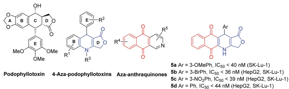
Fig. 1 Structure of podophyllotoxin derivatives, aza-antraquinones derivatives and podophyllotoxin-naphthoquinone compounds (5a, 5d).
