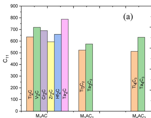
Fig. 17 (a) Calculated elastic constant values for various MXenes. (b) MXene stress–strain curves for \text{Ti}_2\text{C} , \text{Ti}_3\text{C}_2 , \text{Ti}_4\text{C}_3 . Reproduced from ref. 15 with permission from Springer Nature, copyright 2017.
