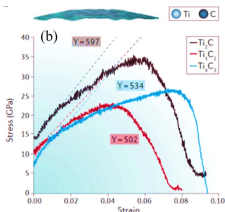
Fig. 17 (a) Calculated elastic constant values for various MXenes. (b) MXene stress–strain curves for \text{Ti}_2\text{C} , \text{Ti}_3\text{C}_2 , \text{Ti}_4\text{C}_3 . Reproduced from ref. 15 with permission from Springer Nature, copyright 2017.
