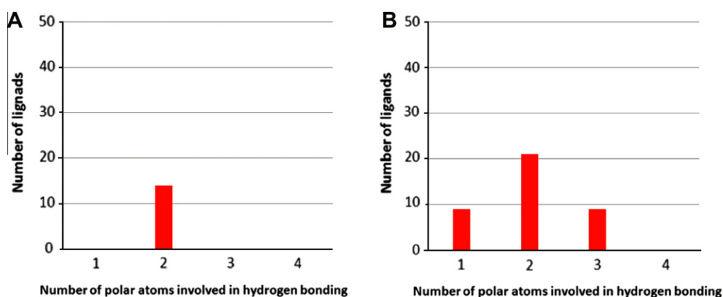
Figure 3. Number of polar interactions formed by: (A) Ligands which docked via the hinge to the apo-structure derived from the ADP-bound structure (PDB ID: 2CN5) (B) Ligands which docked via the mediating water molecule to the apo-structure derived from the NSC-109555-bound structure (PDB ID: 2W0J).
