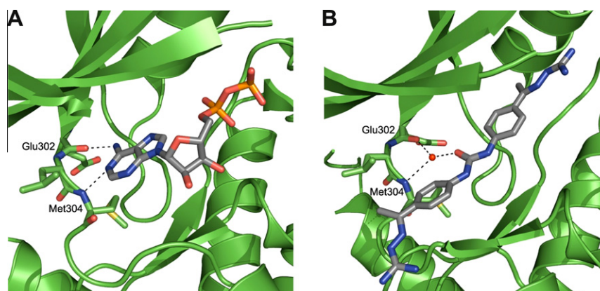
Figure 2. Binding of (A) ADP to CHK2 (PDB ID: 2CN5) 42 and (B) NSC109555 to CHK2 (PDB ID: 2W0J). 43 Hydrogen bonds between the ligand and the hinge region are indicated with black dashed lines.
