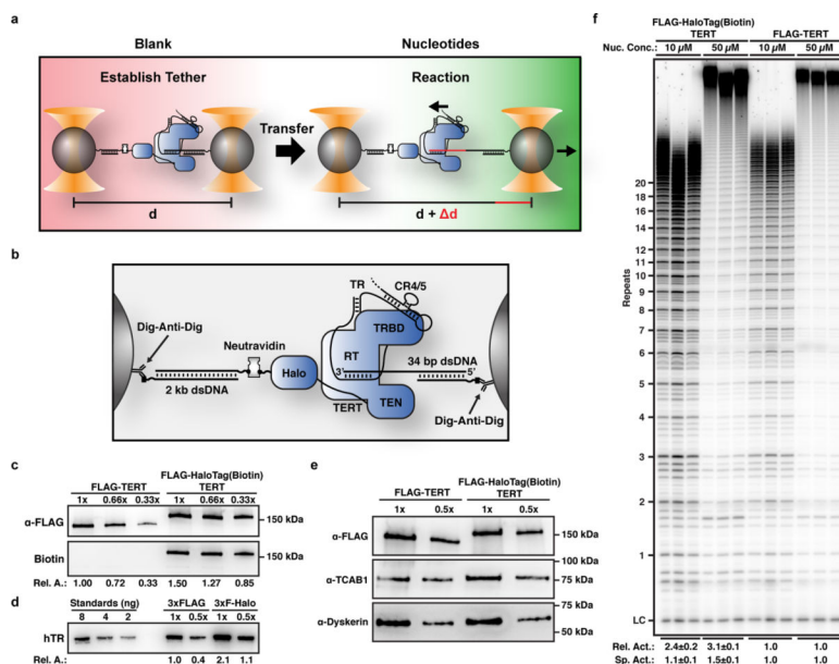
Figure 1. A single-molecule telomerase extension assay using high-resolution dual-trap optical tweezers.
