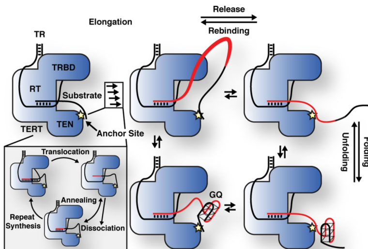
Figure 6. Model for processive telomerase catalysis.
