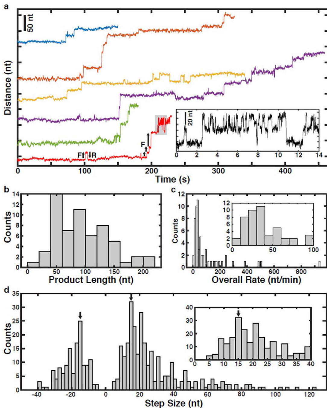
Figure 2. Telomerase releases multiple telomeric repeats in a single step.
