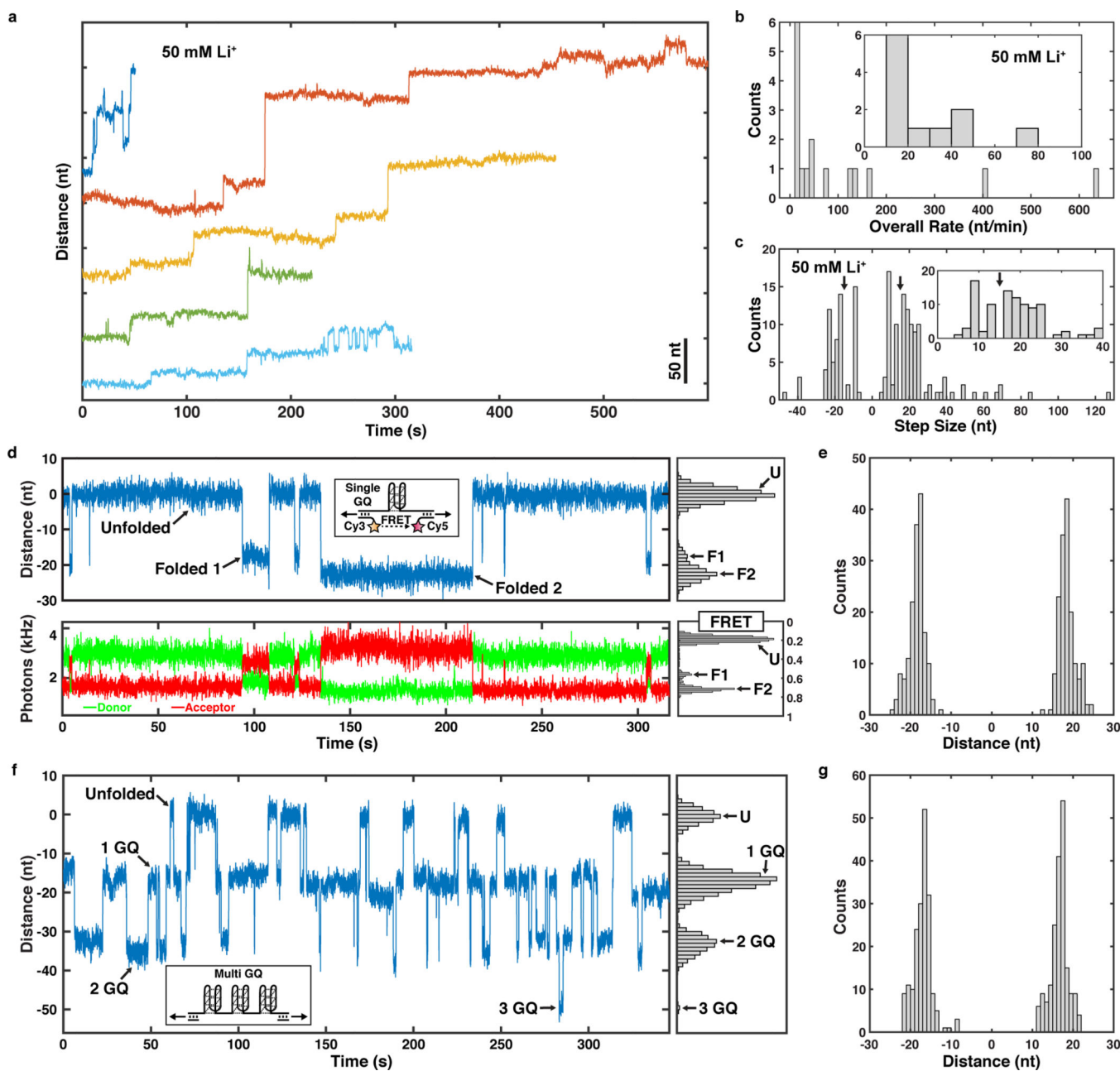
Figure 4. Analysis of telomerase catalysis in the presence of LiCl.
