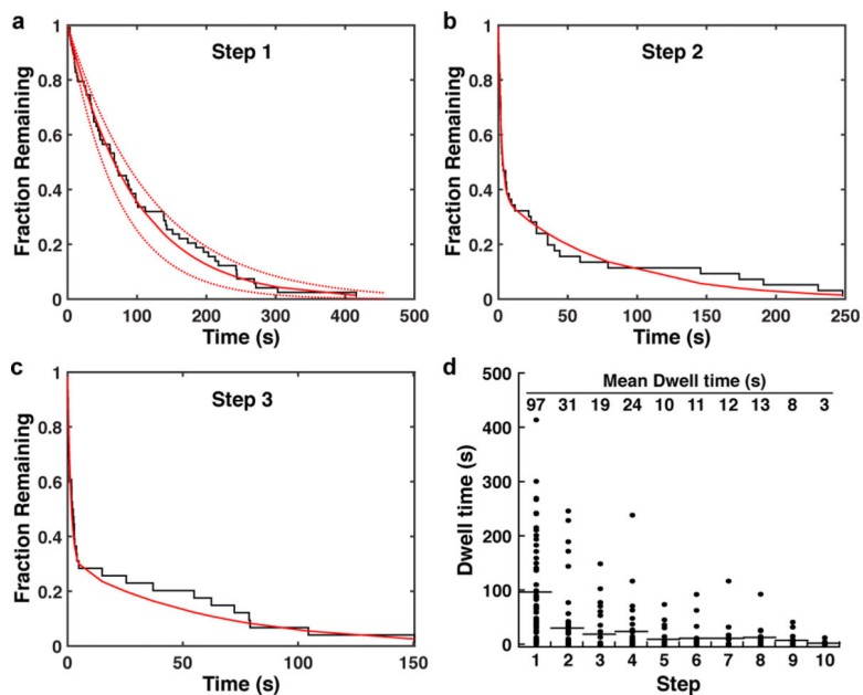
Figure 5. Dissociation from the anchor site controls product release by telomerase. a-c , Inverse cumulative distribution of dwell times for the a first, b second, and c third step of all telomerase trajectories (black staircase, n = 60 traces). Solid red line indicates a single ( a ) or double ( b,c ) exponential fit, dashed lines the 90% confidence intervals. d , Dot plot of individual dwell times for the first 10 steps of all telomerase trajectories ( n = 60 ). Mean dwell time is indicated at the top of the graph and by the black horizontal lines.
