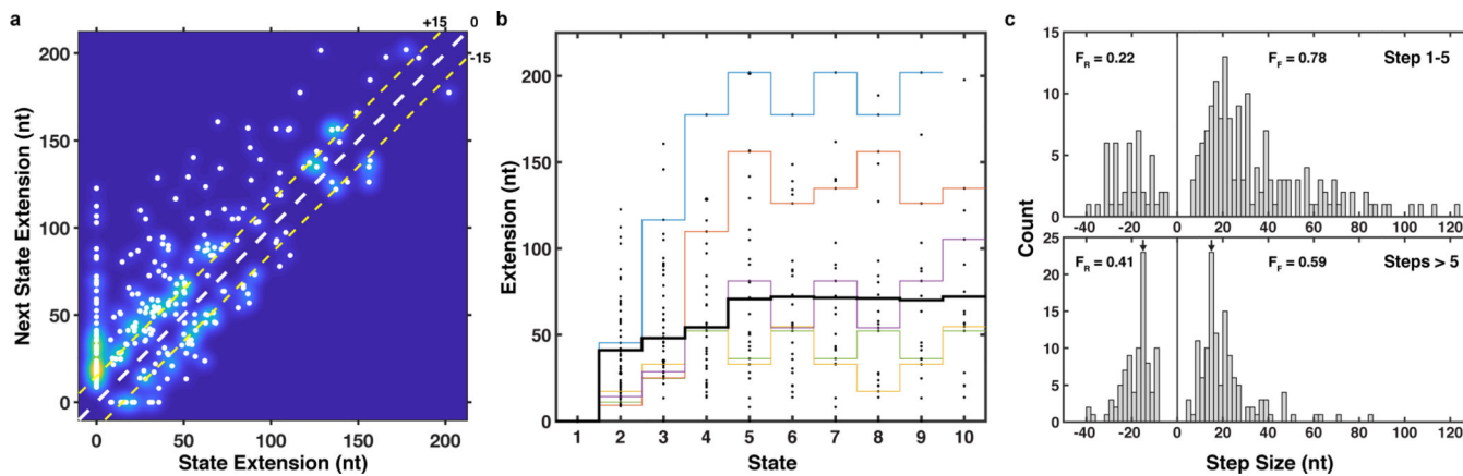
Figure 3. Analysis of processive DNA synthesis and product release by telomerase.
