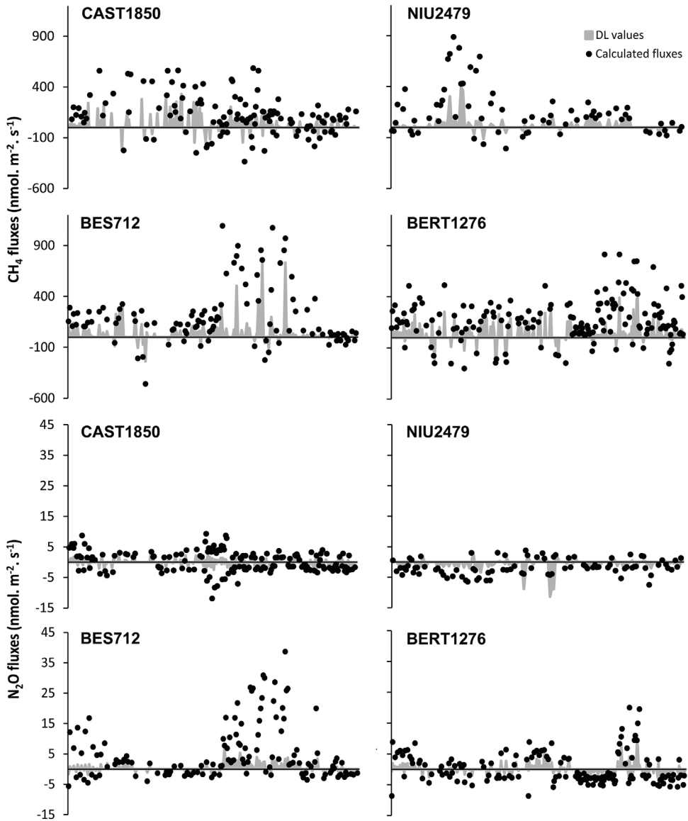
Fig. 6. Comparison between the total calculated CH 4 and N 2 O fluxes and the detection limit values (DL; gray-shaded area) in the four grassland sites along time, along the altitudinal gradient: Besora (BES712), La Bertolina (BERT1276), Castellar de n'Hug (CAST1850), Niu de l'Àliga (NIU2479).
