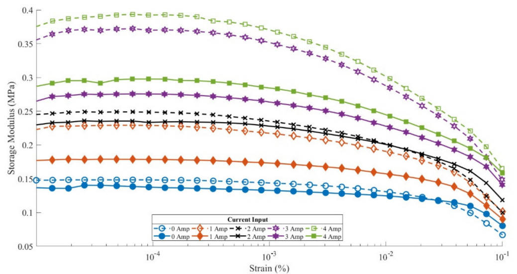
Figure 4. Results of MRE sample rheometer test for anisotropic treated and isotropic untreated.
