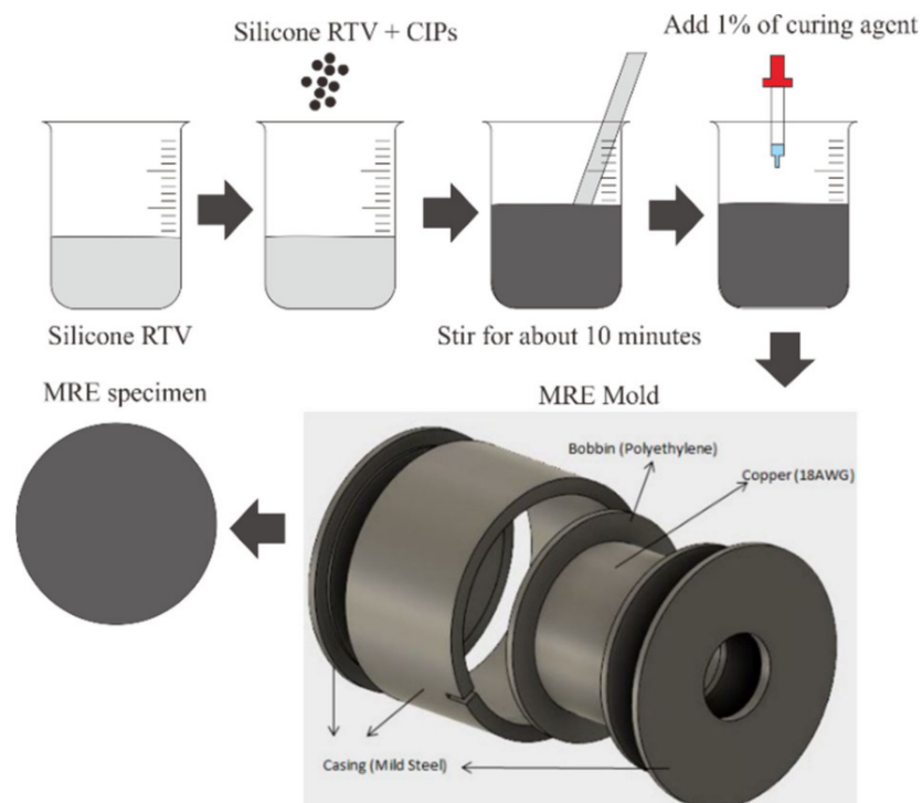
Figure 1. MRE sample preparation.
