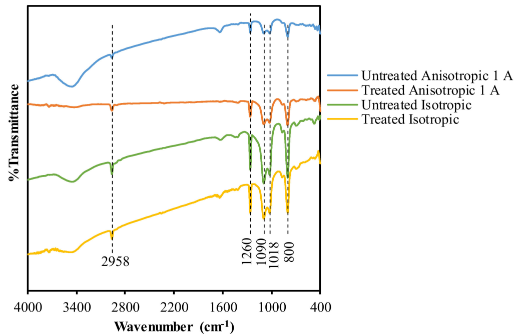
Figure 5. FTIR results.
