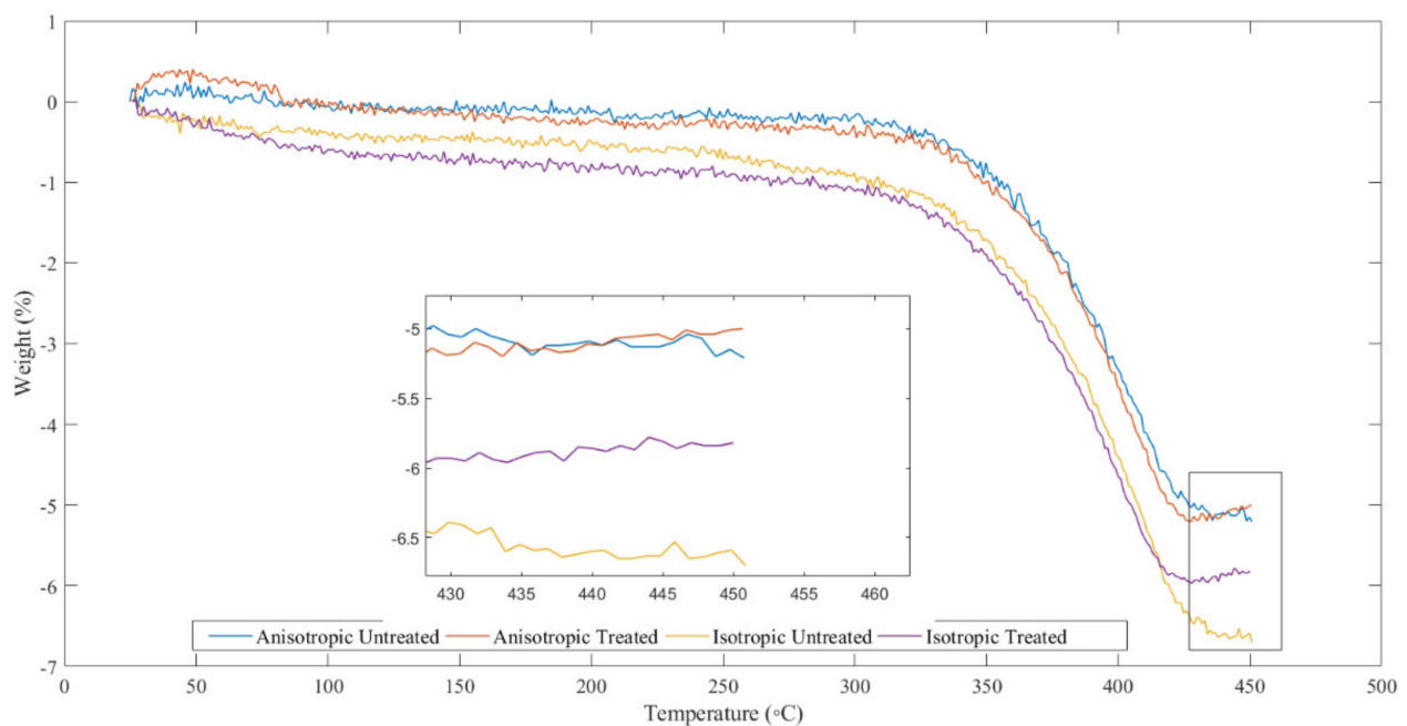
Figure 8. Thermogravimetric curves of MRE specimens.
