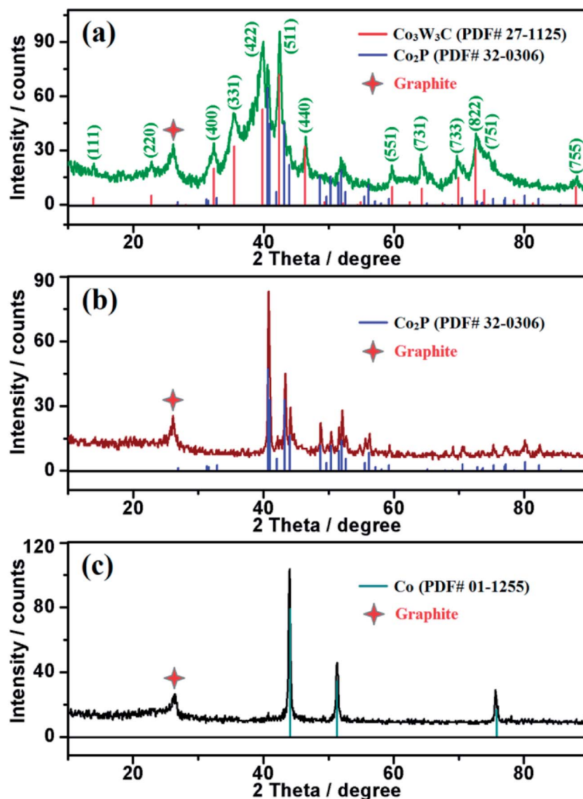
Fig. 1 XRD (a) \text{Co}_3\text{W}_3\text{C}/\text{NPG} (containing \text{Co}_2\text{P} ), (b) NPG (containing \text{Co}_2\text{P} ) and (c) NG (containing Co).
