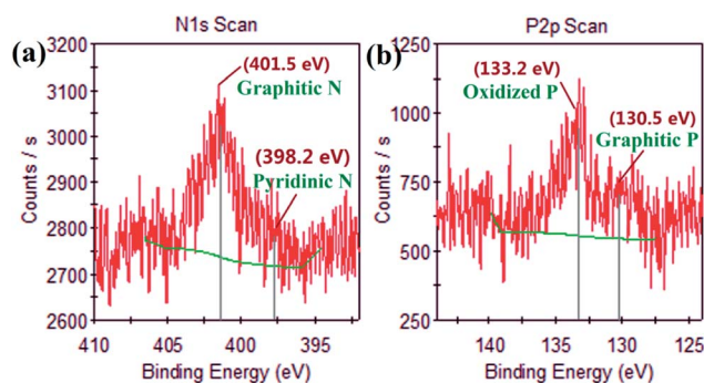
Fig. 2 (a) N1s and (b) P2p XPS spectrum of \text{Co}_3\text{W}_3\text{C}/\text{NPG} .
