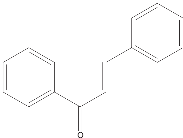
Figure 1 Chalcone backbone.
