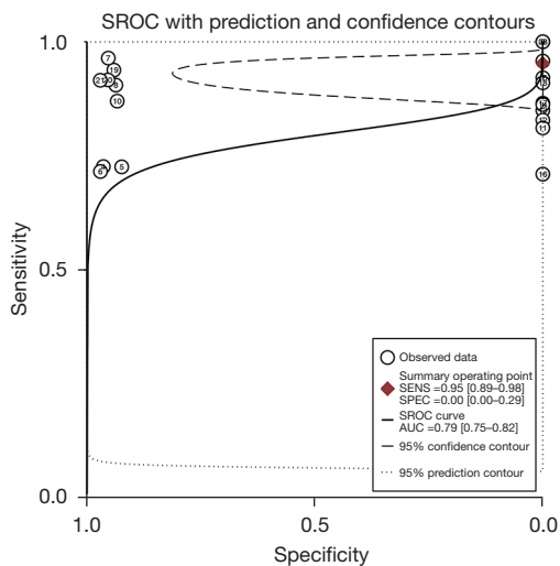
Figure 5 SROC curve of AI-assisted polyp detection. SROC, summary receiver operating characteristic curve; AI, artificial intelligence.
