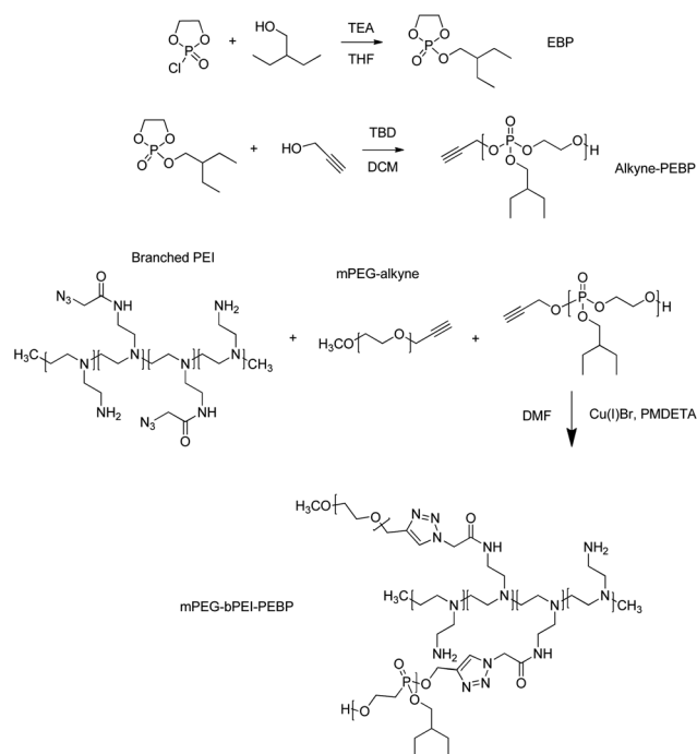
Fig. 2 Synthesis of 2-ethylbutyl phospholane (EBP), alkyne-poly(2-ethylbutyl phospholane) (alkyne-PEBP), and mPEG-bPEI-PEBP copolymer. TEA, triethylamine; THF, tetrahydrofuran; DMAP, dimethylaminopyridine; TBD, 1,5,7-triazabicyclo[4.4.0]dec-5-ene; DCM, dichloromethane; PEI, polyethyleneimine; mPEG, monomethoxypolyethylene glycol; DMF, dimethyl formamide; PMDETA, N,N,N',N',N'' -pentamethyldiethylenetriamine; mPEG-bPEI-PEBP, poly(ethylene glycol)-arsenic-retinoic acid.
