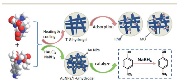
Fig. 1 Schematic of adsorption of the T-G hydrogel and the catalysis of the AuNP/T-G hydrogel.
