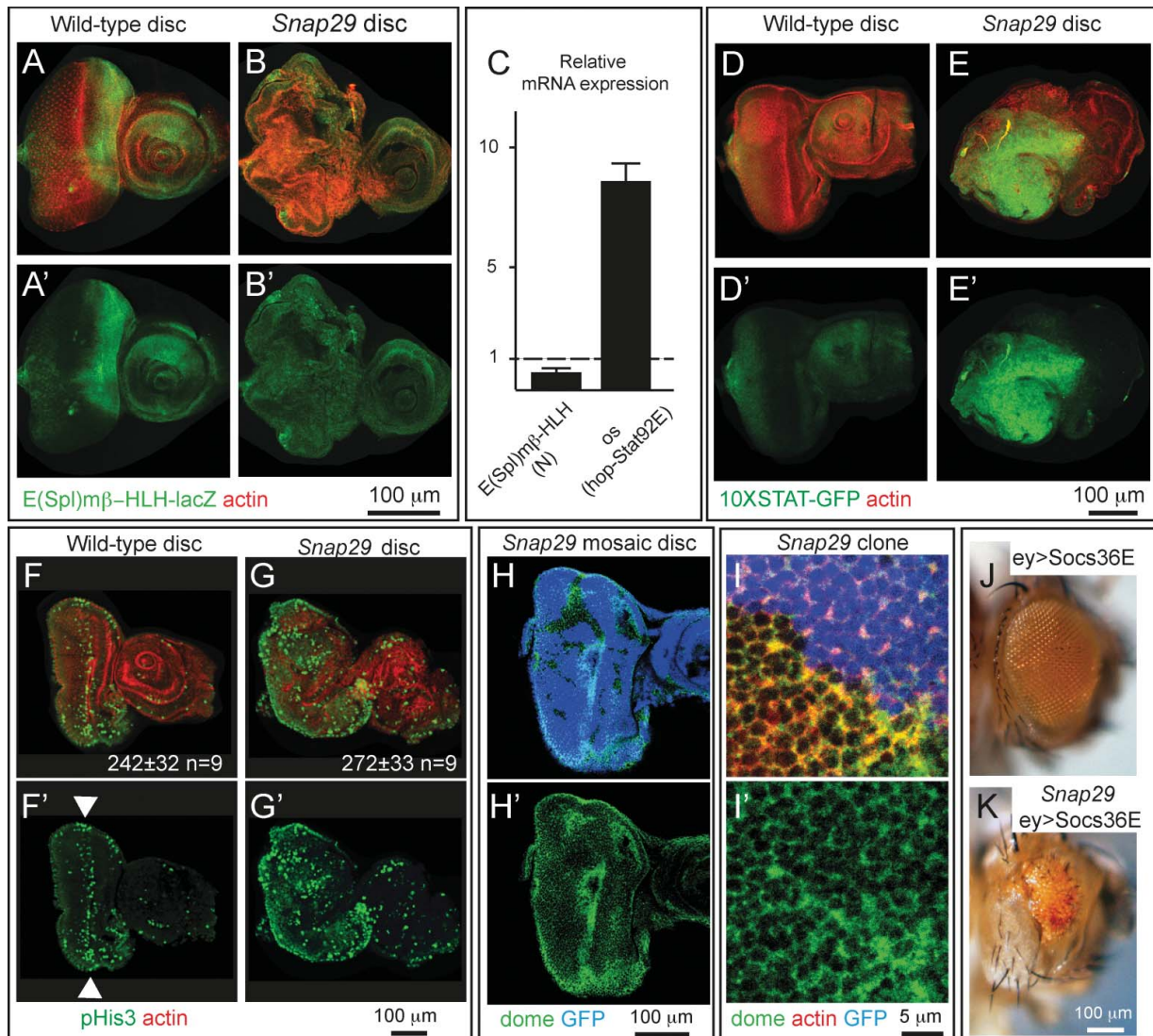
Figure 8. Elevated hop-Stat92E signaling contributes to altered development of Snap29 mutant eye discs. (A and B) WT and Snap29 mutant eye discs expressing E(Spl)mβ-HLH-lacZ, a N signaling reporter, stained as indicated. Snap29 mutant discs display a reduction of N signaling compared to WT. A' and B' show single anti-β-Gal channels. (C) Expression of the indicated signaling target genes in eye disc extracts. The mRNA of a N target is decreased in Snap29 mutant eye-antennal disc extract, while the mRNA of the hop-Stat92E ligand os is greatly elevated, compared to WT. (D and E) The expression of the hop-Stat92E reporter gene 10XSTAT-GFP is increased in mutant discs compared to WT discs. D'-E' are the single GFP channels. (F and G) WT and Snap29 mutant eye-antennal discs stained with anti-phospho-HistoneH3 (pHis3) to detect dividing cells. Compared to WT tissue in which proliferation is mostly limited to the differentiating photoreceptors along the morphogenetic furrow (arrowheads), mutant eye discs display areas containing several pHis3-positive cells, suggesting that mutant cells overproliferate. The average number of pHis3-positive cells in samples of the indicated genotype is indicated. P value (Wilcoxon-Mann Whitney Test) is 0.0625. F'-G' are the single pHis3 channels. (H and I) Clones of Snap29 mutant cells in a mosaic eye discs stained as indicated. Compared to WT (GFP-positive) cells, mutant cells accumulate dome, mostly at the cell cortex. H' and I' shows single dome channels. (J and K) Adult eyes of flies of the indicated genotypes. Eye specific ectopic expression of Socs36E, a hop-Stat92E signaling inhibitor does not impair eye development (J). Socs36E expression in Snap29 mutant eye discs rescues in part eye development and yields adults with reduced eyes (K). In (K), mutant cells expressing the Socs36E give rise to orange photoreceptors, while the few WT cell to the dark red ones.
