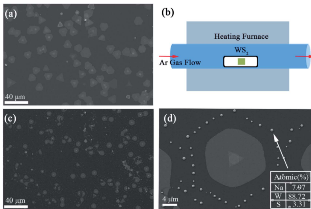
Fig. 1 (a) and (c) SEM images of 2D WS 2 film before and after annealing at 800 °C for 5 minutes (Ar gas flow rate \sim 150 sccm). (b) Schematic of the thermal annealing for WS 2 film. (d) is a high magnification SEM image of (c) with the EDS result of the granule.
