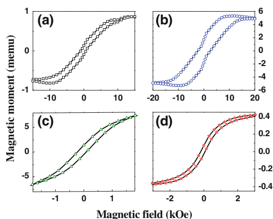
Fig. 4 Magnetic hysteresis loop for 50-nm thermally evaporated nickel thin film for a untreated as deposited, b electric field treated at 2 kV/cm, c excimer laser treated at 0.5 J/cm 2 and d trench-template assisted technique
