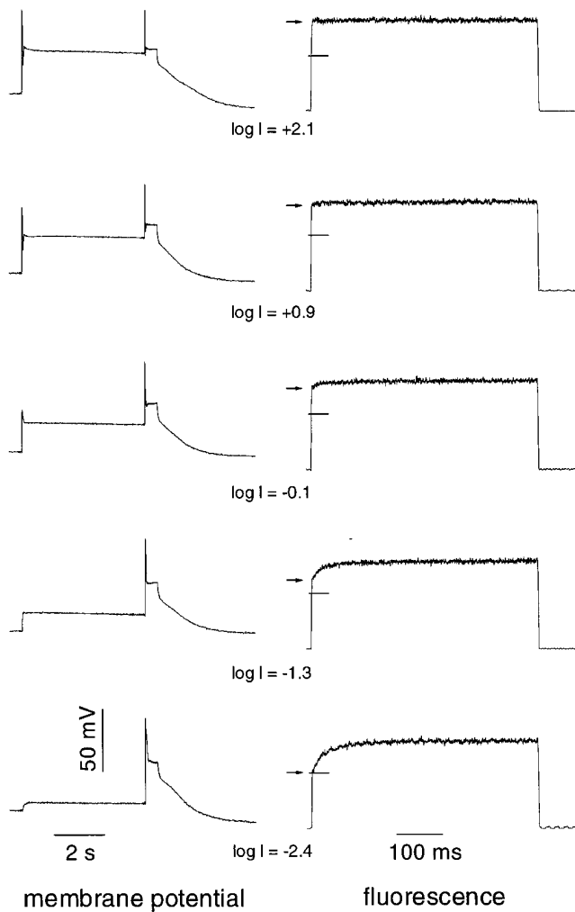
FIGURE 5. Example of the double pulse experiments used to determine Ca_i as a function of light intensity. Membrane potential traces are given in the left hand column. The dye-injected (OG1) and dark-adapted cell was stimulated with an adapting light (5 s), the intensity of which is indicated for each experiment. Intensities are expressed relative to the light intensity that caused a half maximal peak depolarization; this intensity was assigned the value \log I = 0 . After adapting for 5 s, the level of Ca_i was probed with a bright test flash (500 ms). The fluorescence signal measured during this test flash is shown in the right-hand column on an expanded time scale. The horizontal line at the beginning of the fluorescence traces indicates the initial fluorescence value when no adapting light was given. With increasing adapting intensity, the initial value of the fluorescence (arrows) increases. At the highest adapting intensities used, no increase in fluorescence can be observed during the test flash due to saturation of the high affinity dye OG1. All traces shown are averages of five recordings.
