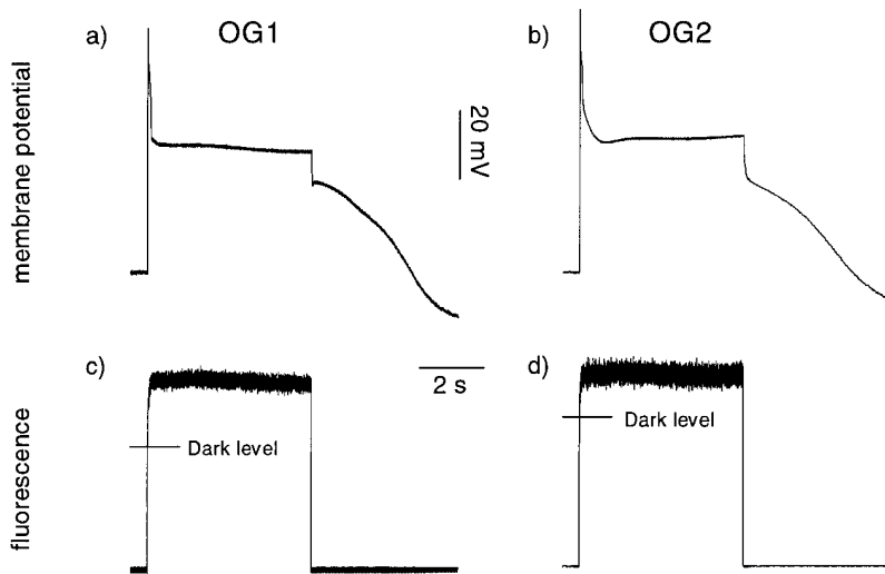
FIGURE 4. Membrane potential ( a and b ) and fluorescence ( c and d ) signals from two cells injected with the high affinity dyes OG1 ( a and c ) and OG2 ( b and d ), respectively. The dark-adapted cells were illuminated for 5 s with light of saturating intensity. The fluorescence signal increases monotonically upon stimulation and does not display the peak that can be seen when using the low affinity dye OG5N (Fig. 2). This indicates that the high affinity dyes OG1 and OG2 are saturated by the levels of Ca_i reached under bright illumination. This implies that in these conditions Ca_i exceeds 10 \mu\text{M} , the concentration where OG2 saturates (Haugland, 1996). Traces in a and c are averages of five recordings, traces in b and d are averages of seven recordings.
