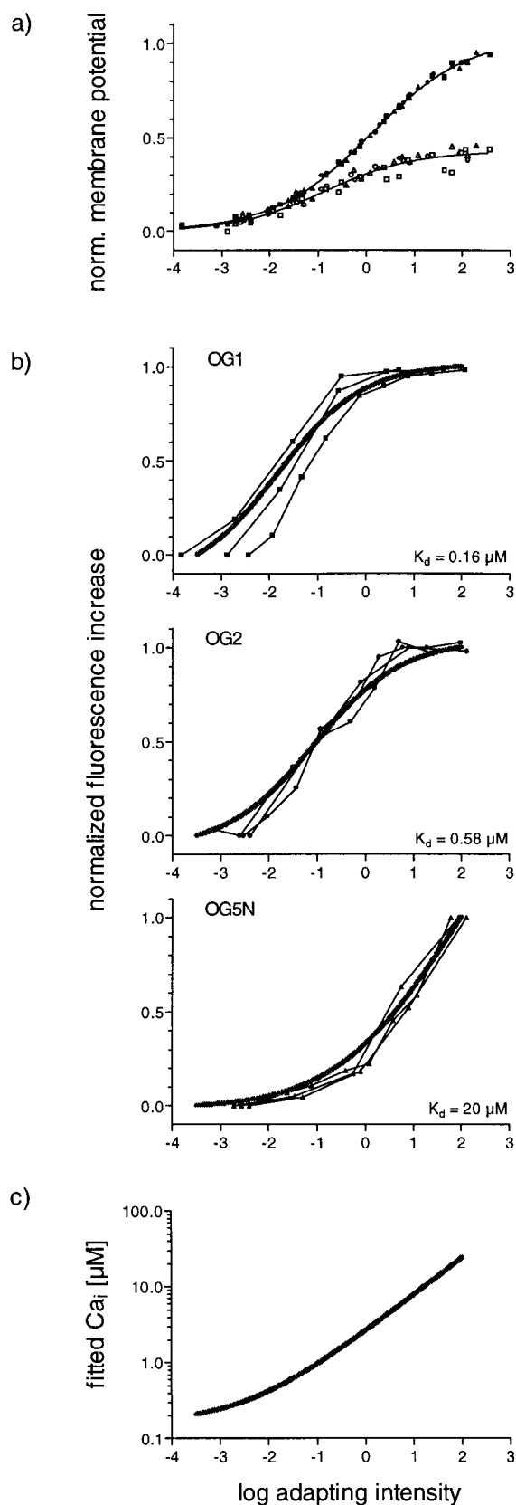
FIGURE 6. Summary of the double pulse experiments. (a) Normalized depolarization of the peak (filled symbols) and plateau (open symbols) of the membrane potential are given as a function of
