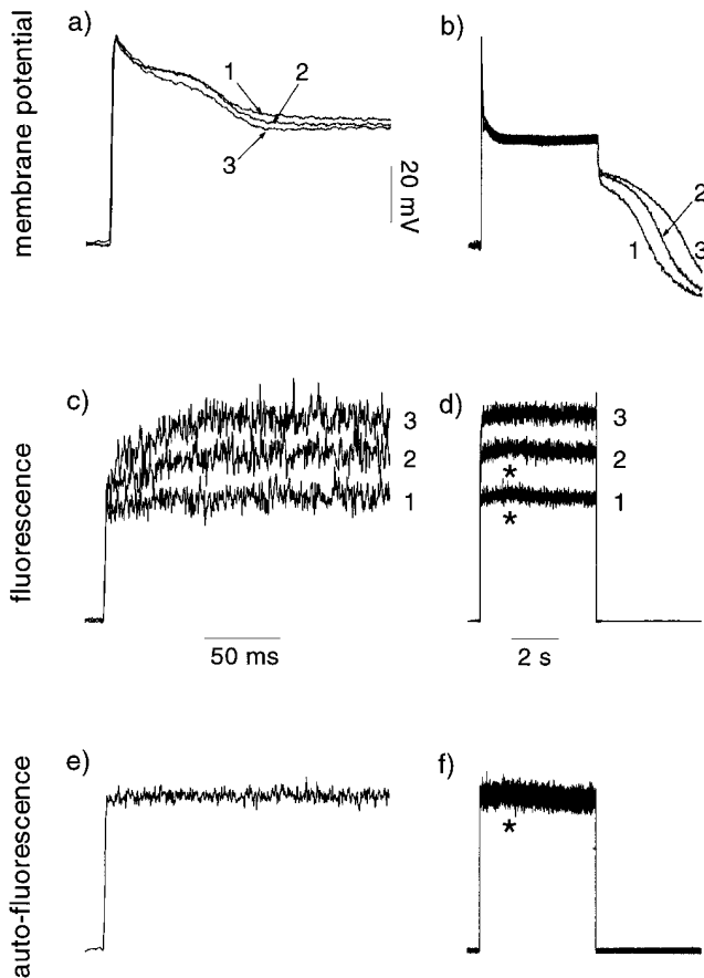
FIGURE 3. The effects of dye filling on the membrane potential. The photoreceptor cell was impaled with an electrode containing OG2 and then filled without applying current. Traces 1–3 were measured 1, 4, and 6 min, respectively, after impalement by a 5-s stimulus of saturating intensity. While the fluorescence signal ( c and d ) increases with time of impalement, indicative for an ongoing dye-loading, the membrane potential response ( a and b ) of the cell during the light stimulus is hardly changed. Only after turning the stimulus off can a distinct prolongation of the depolarizing after-potential be seen, due to an increase in the concentration of the dye ( b ). The fluorescence traces in d are smoothed by adjacent averaging with a window size of 20 sample points (equivalent to 4 ms) and therefore the rising phase that is visible in c is not discernible in d . The traces in e and f were obtained from a different preparation in which no cell had been dye-filled; these traces are averages of five recordings. They show that the tissue autofluorescence is essentially constant, except for a small, transient increase in fluorescence signal (*) that can be attributed to a light-induced change in redox state of mitochondrial flavoproteins (Stavenga and Tinbergen, 1983).
