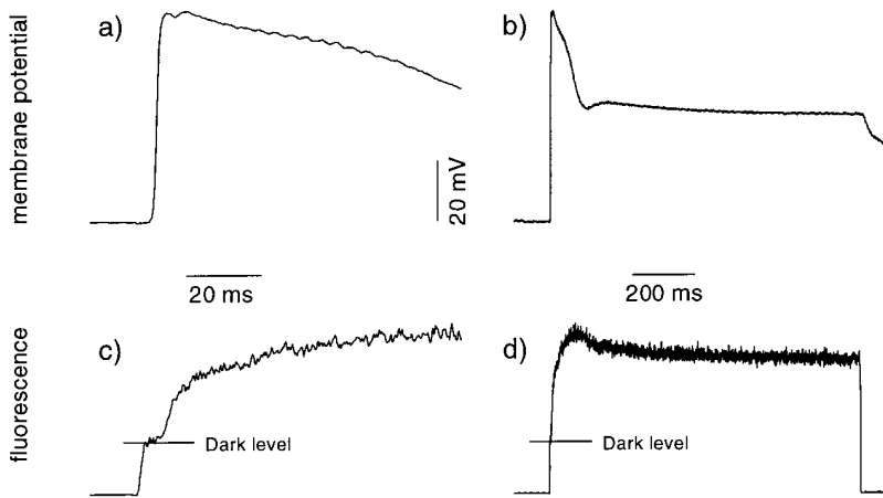
FIGURE 2. Simultaneous recording of membrane potential ( a and b ) and \text{Ca}^{2+} -induced fluorescence ( c and d ) from a dark-adapted photoreceptor illuminated with saturating light. The same data are shown with high ( a and c ) and low ( b and d ) temporal resolution. The cell was injected with the low affinity dye OG5N. The fluorescence signal increases very fast after opening the shutter and peaks after \sim 100 ms before levelling off towards a plateau. The depolarization of the membrane, however, displays still faster kinetics. All traces are averages of nine recordings.
