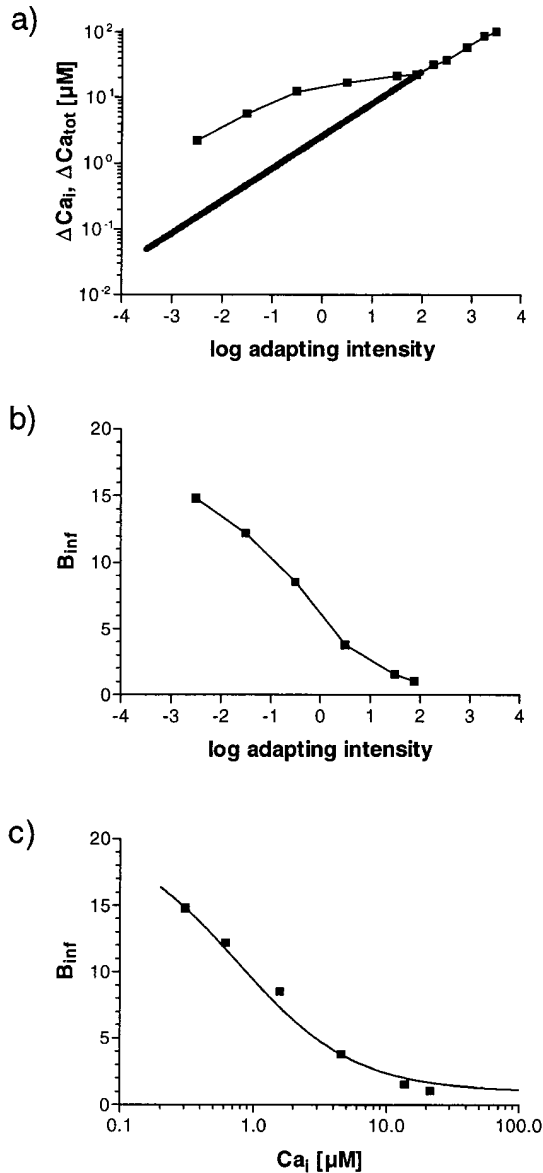
FIGURE 7. (a) Comparison of changes in Ca_i ( \Delta Ca_i = Ca_i - Ca_{i,da} = a * I^b , continuous bold line, taken from Fig. 6 c) and changes in the total Ca^{2+} concentration ( \Delta Ca_{tot} , ■) measured by Sandler and Kirschfeld (1988, their Fig. 1 c). The \Delta Ca_{tot} values were derived using the formula \Delta Ca_{tot} = \Delta Ca_o / R . The ratio R between the volume of the photoreceptors and the extracellular space was assumed to be 6.3 (Sandler and Kirschfeld, 1991), and the change in extracellular Ca^{2+} concentration ( \Delta Ca_o ) was calculated assuming that in the dark-adapted state the extracellular Ca^{2+} concentration amounts to 1.4 mM (Sandler and Kirschfeld, 1991). At \log I = 2 , the two curves approximate each other. At lower intensities, however, \Delta Ca_{tot} values are larger than the values obtained with the dyes. This indicates that the influx of Ca^{2+} is buffered. (b) Buffering coefficient of the Ca^{2+} influx ( B_{inf} = \Delta Ca_{tot} / \Delta Ca_i ) shown as a function of adapting light intensity. (c) Same data plotted as a function of Ca_i . The continuous line was obtained by fitting a simple buffer model (see DISCUSSION). The buffering of the Ca^{2+} influx reduces with increasing Ca_i , and at Ca_i levels above 10 \mu M buffering becomes minimal.
